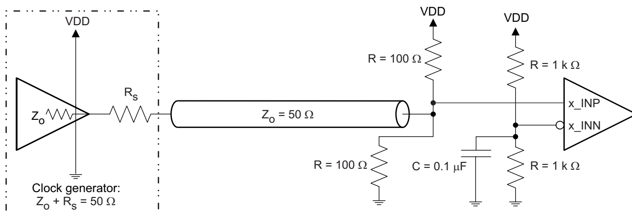
Figure 3. LVCMOS Input DC Configuration During Device Test
