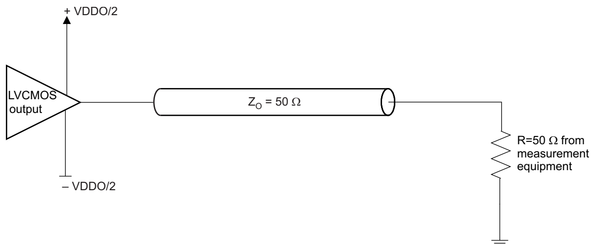
Figure 2. LVCMOS Output DC Configuration; Test Load Circuit
