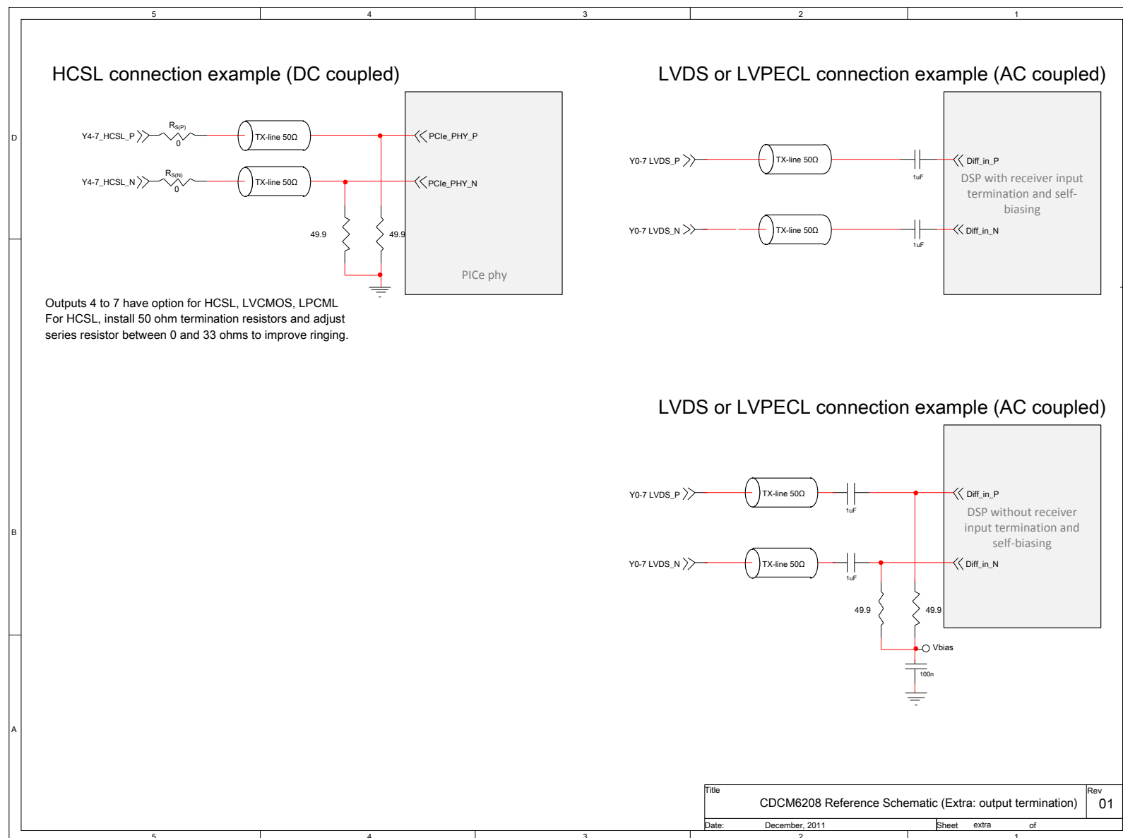
Figure 63. Schematic Page 4
