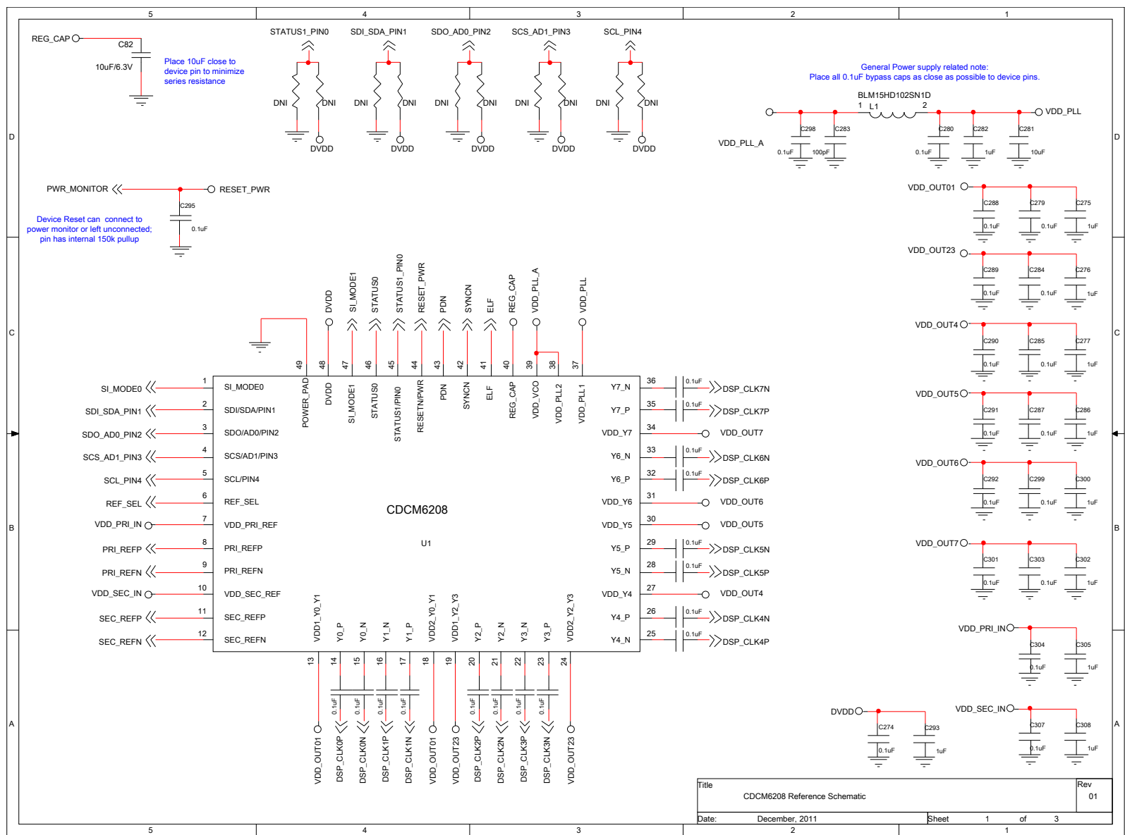
Figure 60. Schematic Page 1
