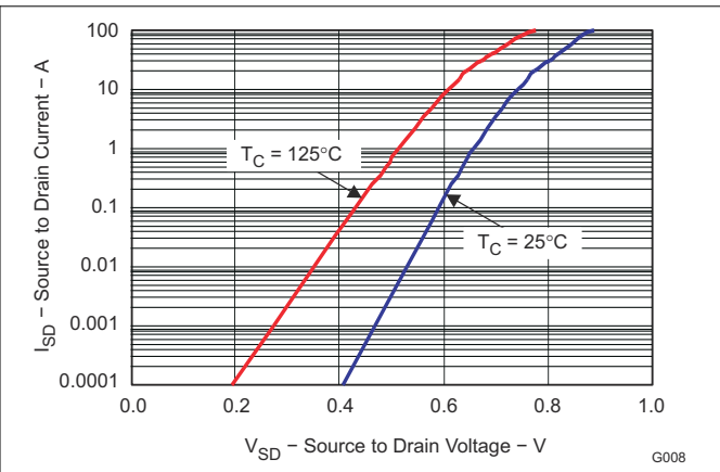
Figure 6-9. Typical Diode Forward Voltage
