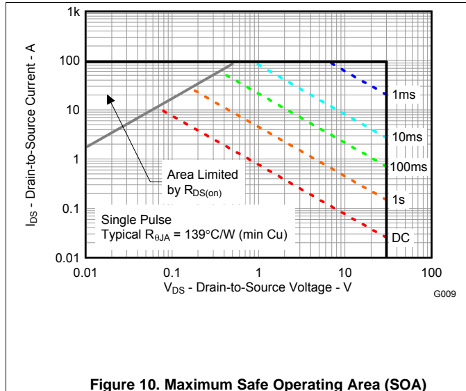
Figure 10. Maximum Safe Operating Area (SOA)
