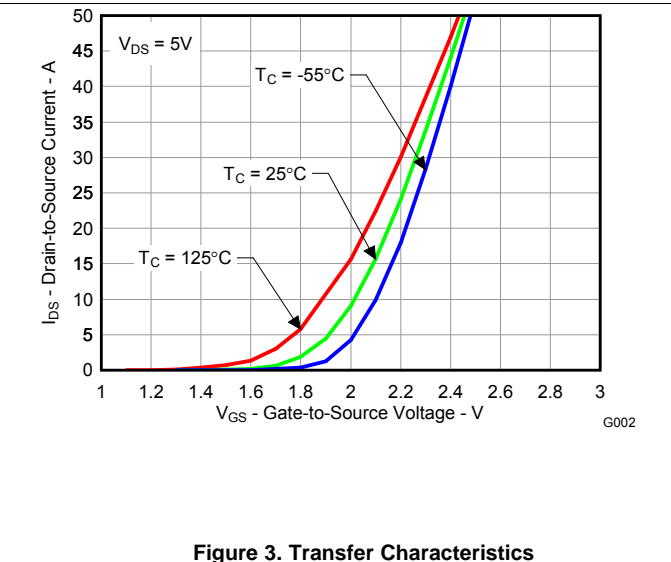
Figure 3. Transfer Characteristics
