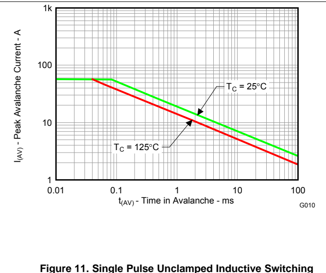
Figure 11. Single Pulse Unclamped Inductive Switching
