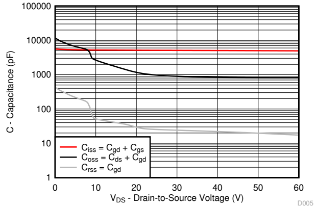
Figure 3-5. Capacitance
