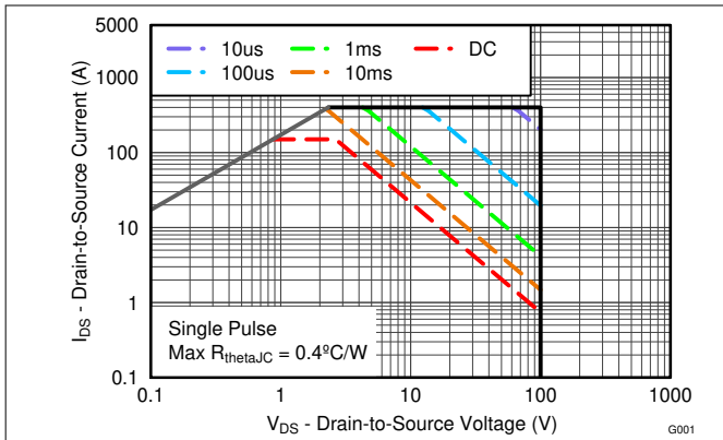
Figure 4-10. Maximum Safe Operating Area
