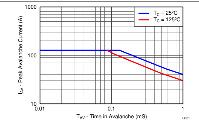
Figure 4-11. Single Pulse Unclamped Inductive Switching
