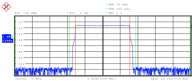
Figure 40. DAC3164 ACPR Four-Carrier WCDMA Test Mode 1
