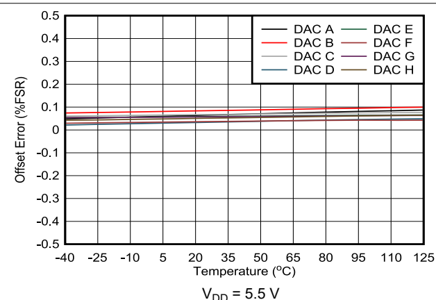
Figure 5-25. Offset Error vs Temperature
