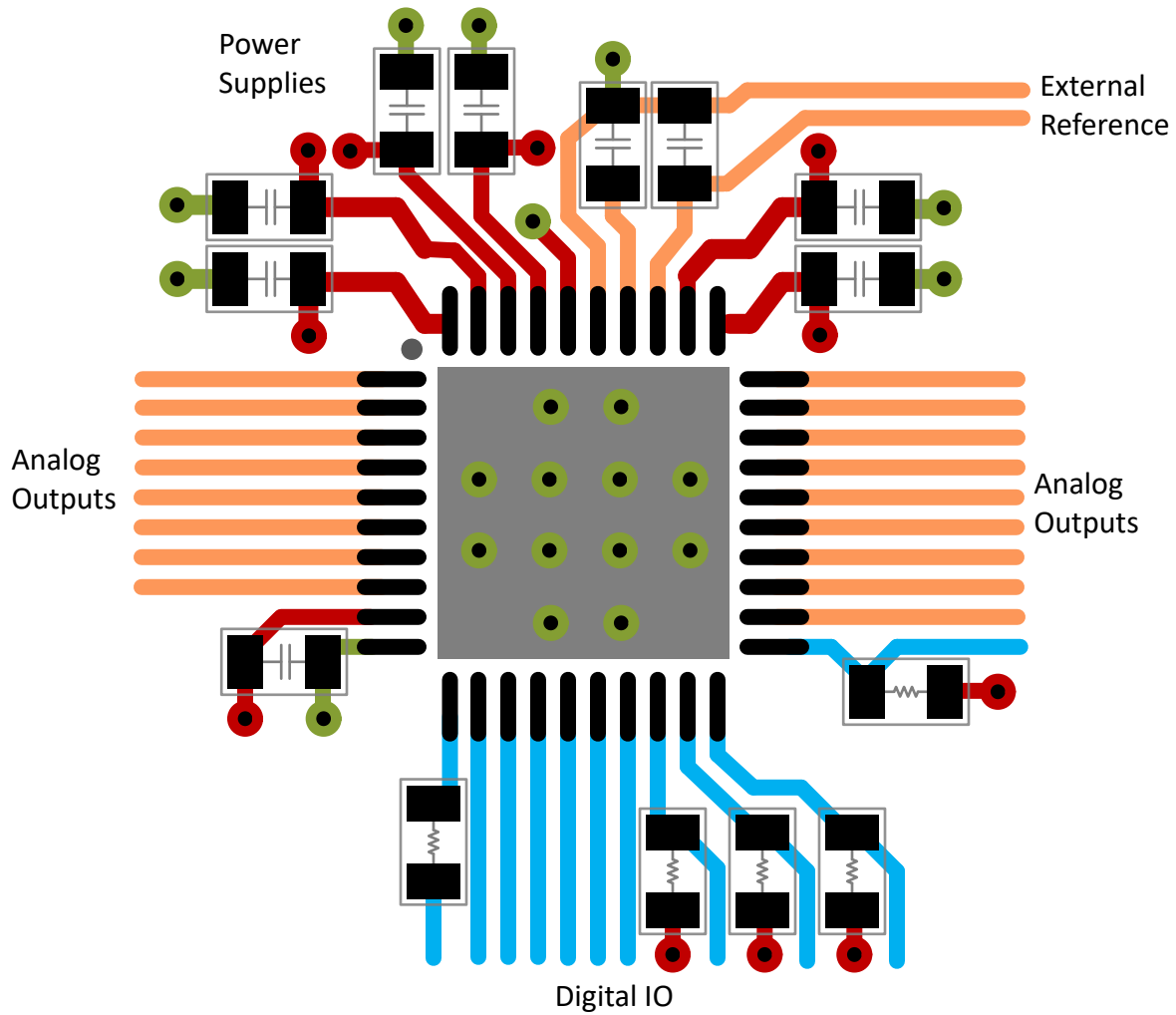
Figure 8-4. Example Layout
