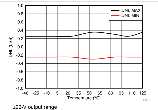
Figure 5-13. Differential Linearity Error vs Temperature
