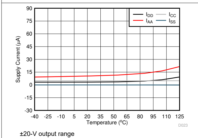
Figure 5-26. Power-Down Current vs Temperature
