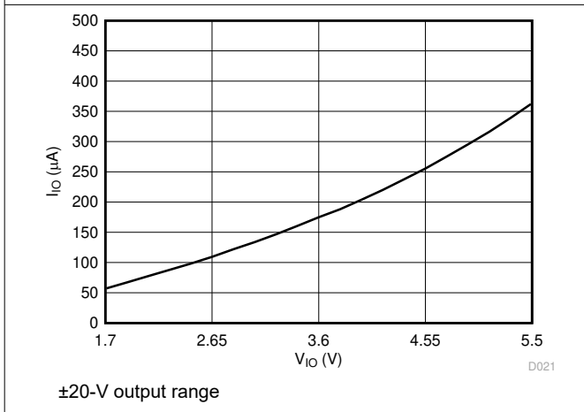
Figure 5-24. Supply Current ( I_{IO} ) vs Supply Voltage
