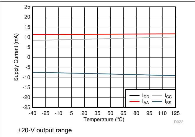
Figure 5-25. Supply Current vs Temperature
