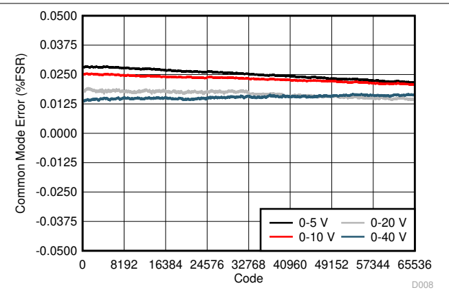
Figure 5-11. Common Mode Error vs Digital Input Code (Differential Unipolar Outputs)
