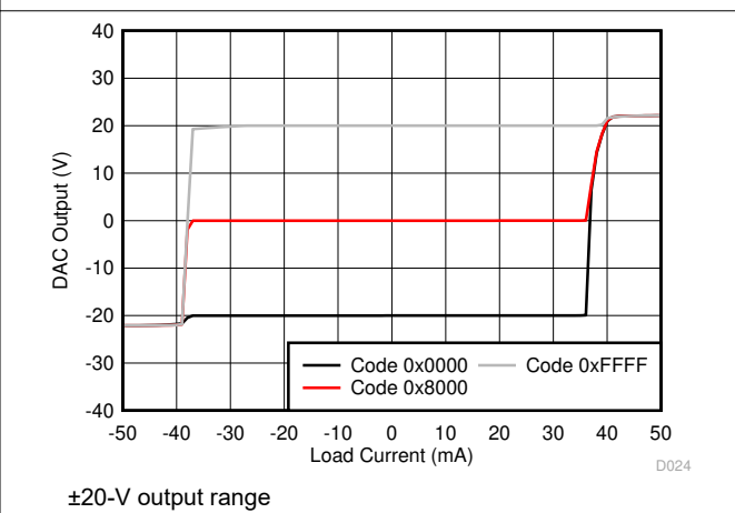
Figure 5-27. Source and Sink Capability
