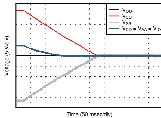
Figure 5-37. Power-Down Response
