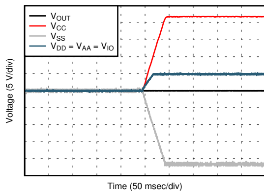
Figure 5-36. Power-Up Response
