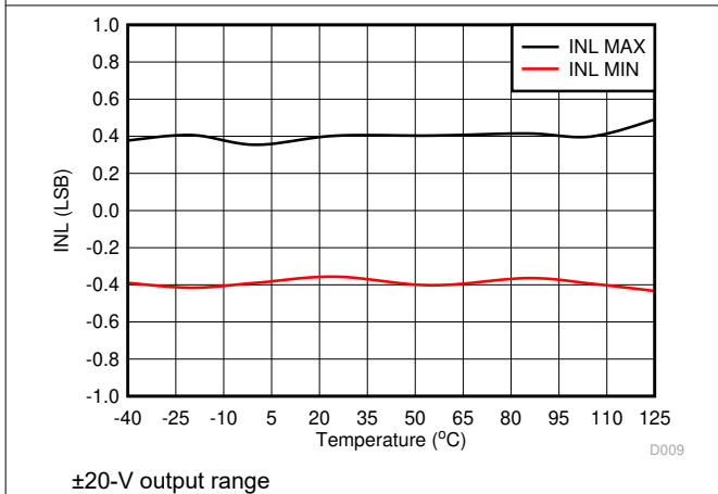
Figure 5-12. Integral Linearity Error vs Temperature
