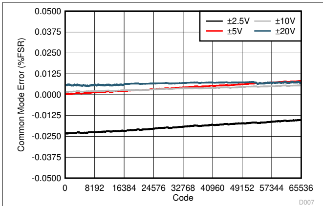
Figure 5-10. Common Mode Error vs Digital Input Code (Differential Bipolar Outputs)
