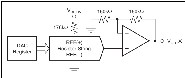
Figure 111. Device Architecture
