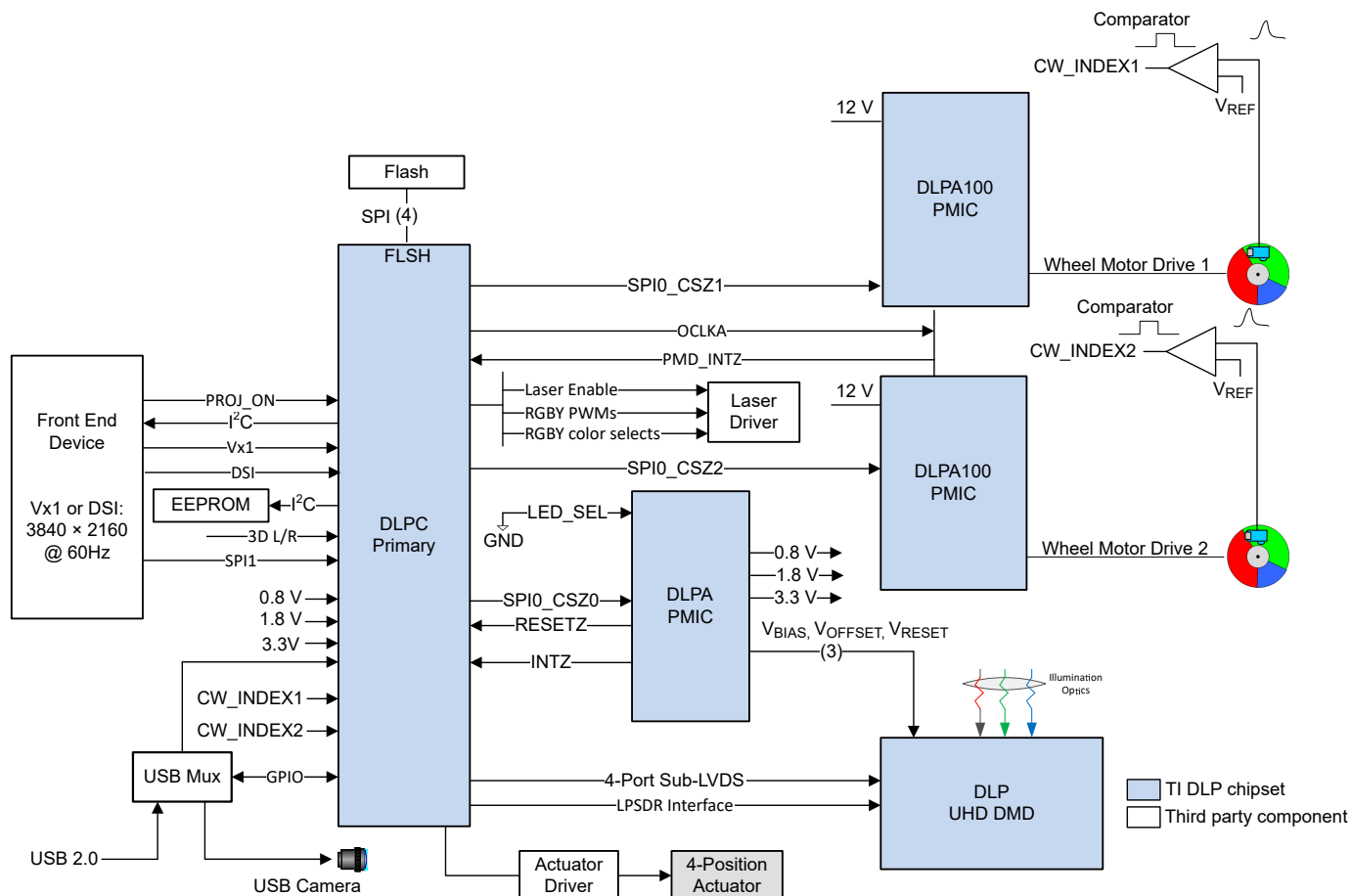
Figure 6-2. Laser-Phosphor Functional Block Diagram
