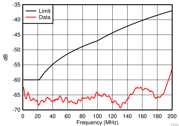
Figure 8-9. MDI Mode Conversion
