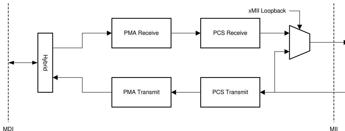
Figure 7-5. xMII Loopback
