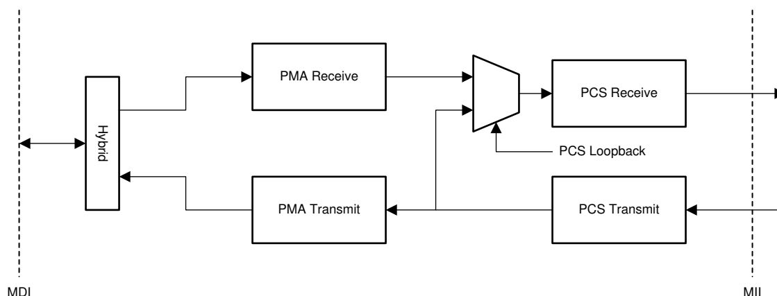
Figure 7-6. PCS Loopback
