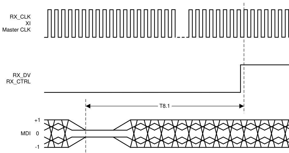
Figure 7-4. Receive Latency
