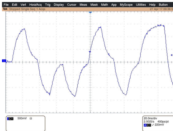
Figure 8-7. MDI IDLE Stream
