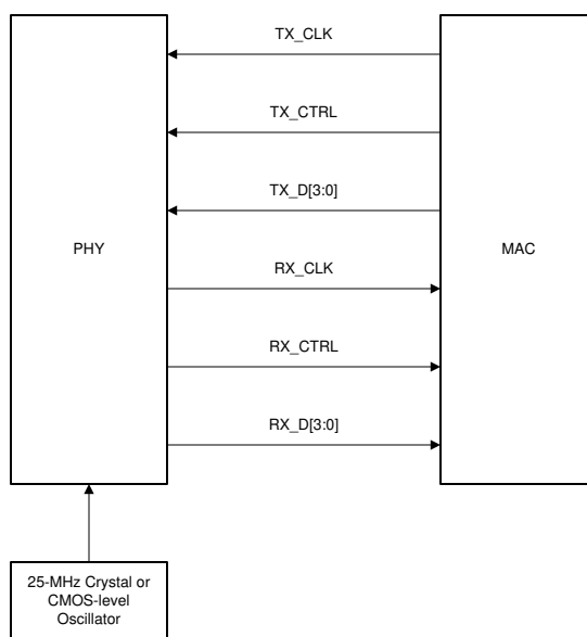
Figure 7-12. RGMII Connections
