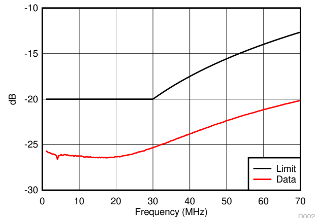
Figure 8-10. MDI Return Loss
