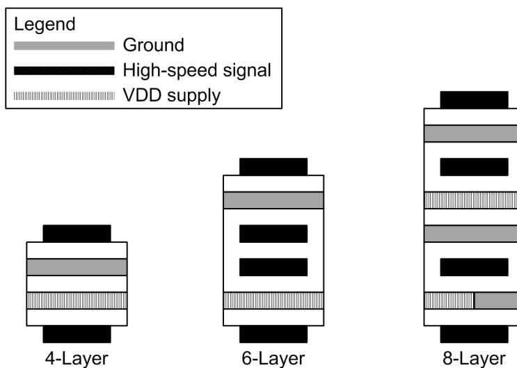
Figure 8-13. Recommended PCB Layer Stack-Up
