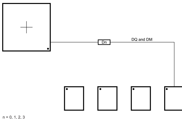
Figure 8-81. DQ/DM Routing With Any Number of Allowed DDR3 Devices
