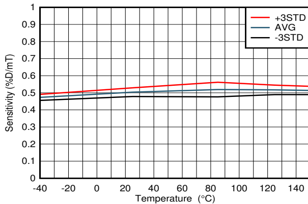
DRV5057Z3, V_{CC} = 5.0 V
