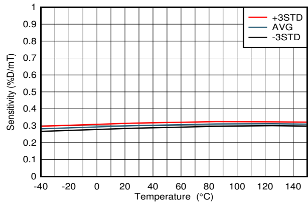
DRV5057Z3, V_{CC} = 3.3 V
