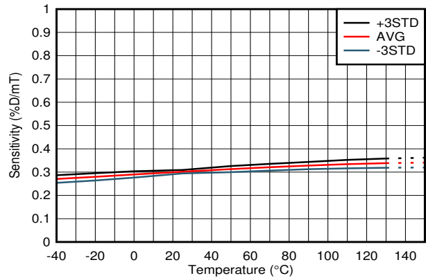
DRV5057A3, V_{CC} = 3.3 V
