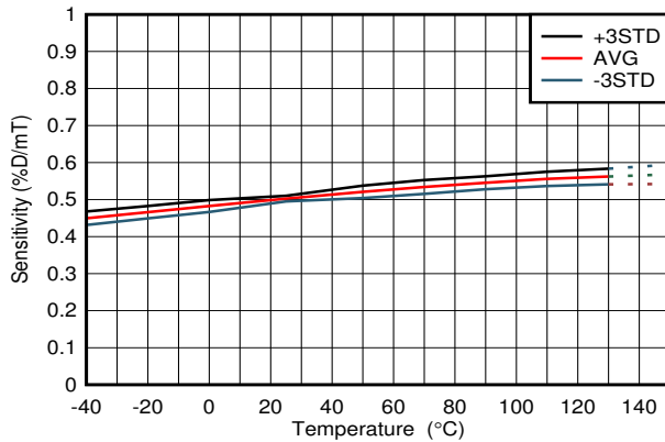
DRV5057A3, V_{CC} = 5.0 V
