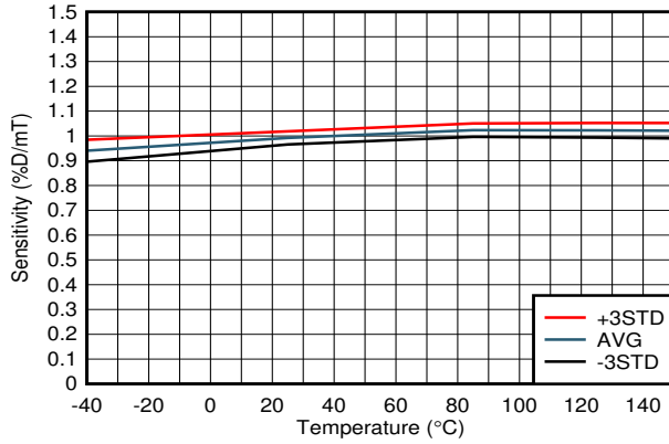
DRV5057Z2, V_{CC} = 5.0 V
