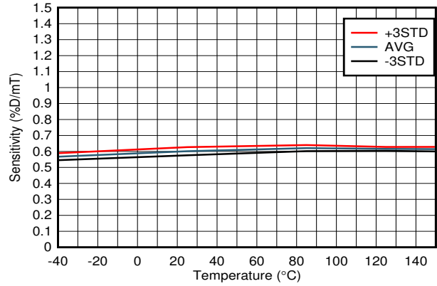
DRV5057Z2, V_{CC} = 3.3 V
