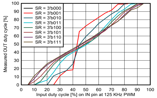
Figure 6-19. Measured Duty Cycle vs Input Duty Cycle at PWM frequency of 125 KHz at V_{VM} = 13.5 V for HS recirculation
