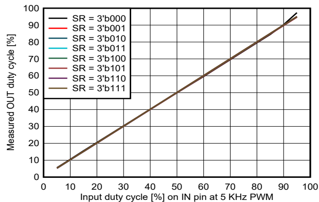
Figure 6-16. Measured Duty Cycle vs Input Duty Cycle at PWM frequency of 5 KHz at V_{VM} = 13.5\text{ V} for HS recirculation
