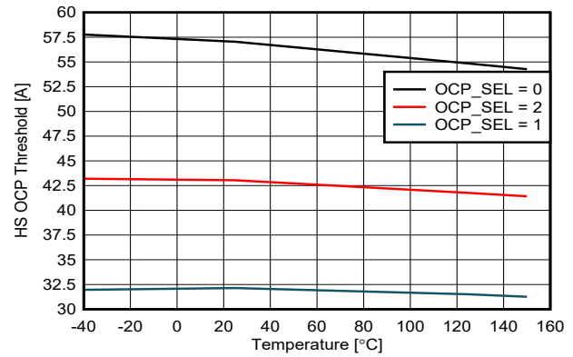
Figure 6-13. HS OCP Threshold vs Temperature at V_{VM} = 13.5\text{ V}
