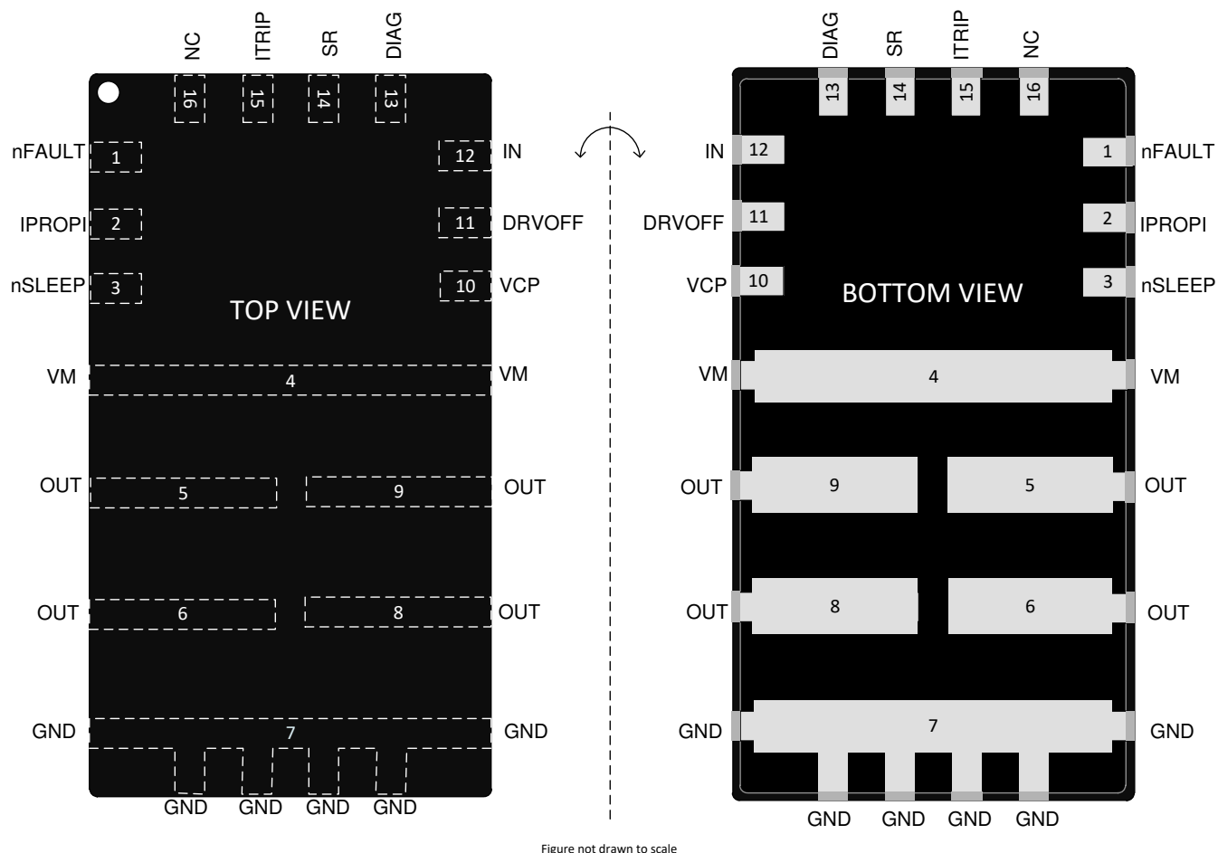
Figure 5-1. DRV8144H-Q1 HW variant in VQFN-HR (16) package
