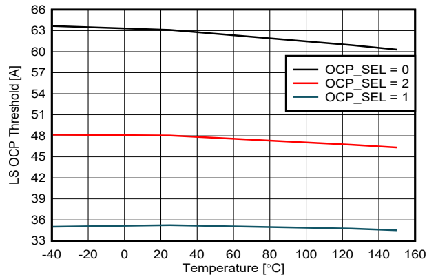
Figure 6-12. LS OCP Threshold vs Temperature at V_{VM} = 13.5\text{ V}
