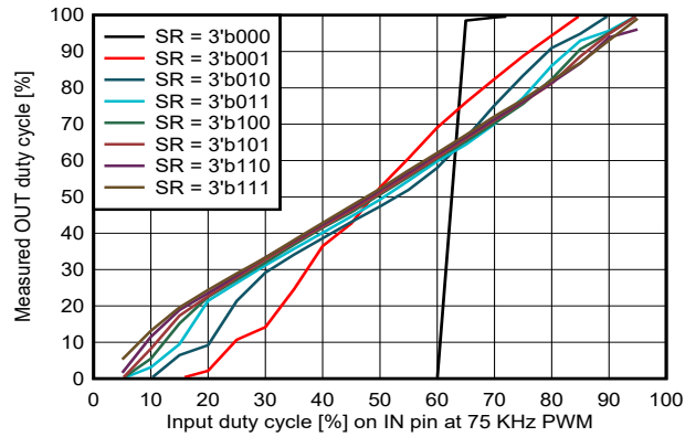
Figure 6-18. Measured Duty Cycle vs Input Duty Cycle at PWM frequency of 75 KHz at V_{VM} = 13.5 V for HS recirculation
