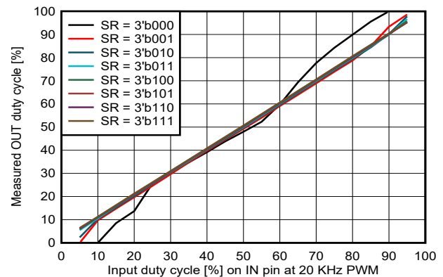
Figure 6-17. Measured Duty Cycle vs Input Duty Cycle at PWM frequency of 20 KHz at V_{VM} = 13.5\text{ V} for HS recirculation
