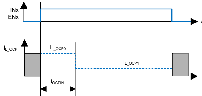
Figure 7-13. Overcurrent Threshold
