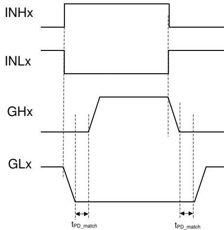
Figure 6-2. Propagation Delay Match (t PD_match )
