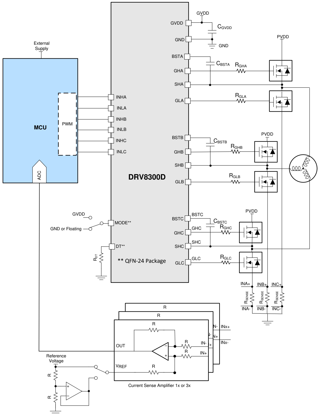
Figure 8-1. Application Schematic
