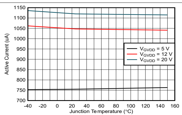
Figure 6-4. Supply Current Over Temperature
