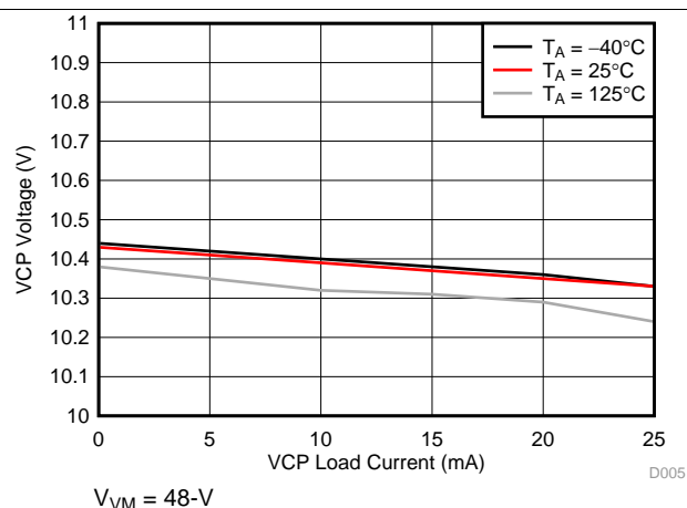
Figure 6. VCP Voltage Over Load
