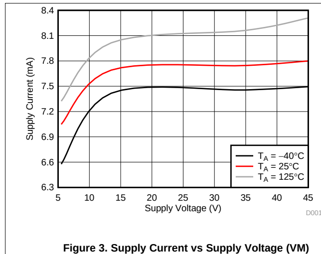
Figure 3. Supply Current vs Supply Voltage (VM)
