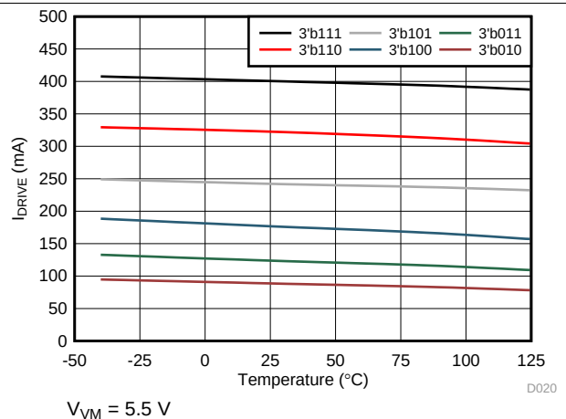
Figure 22. High-Side Sink Current
