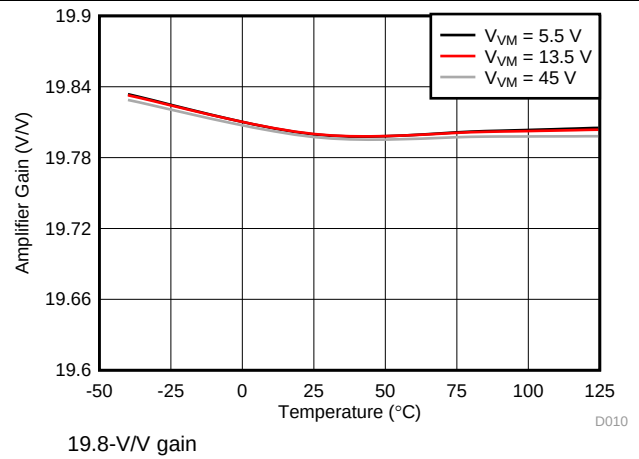
Figure 12. Amplifier Gain
