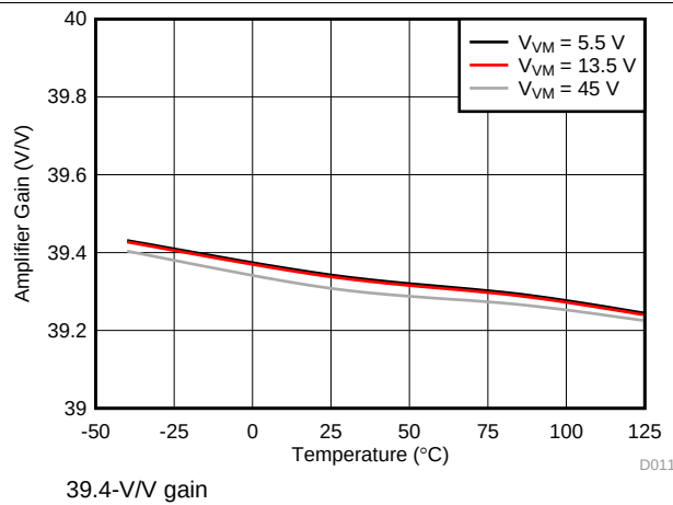
Figure 13. Amplifier Gain
