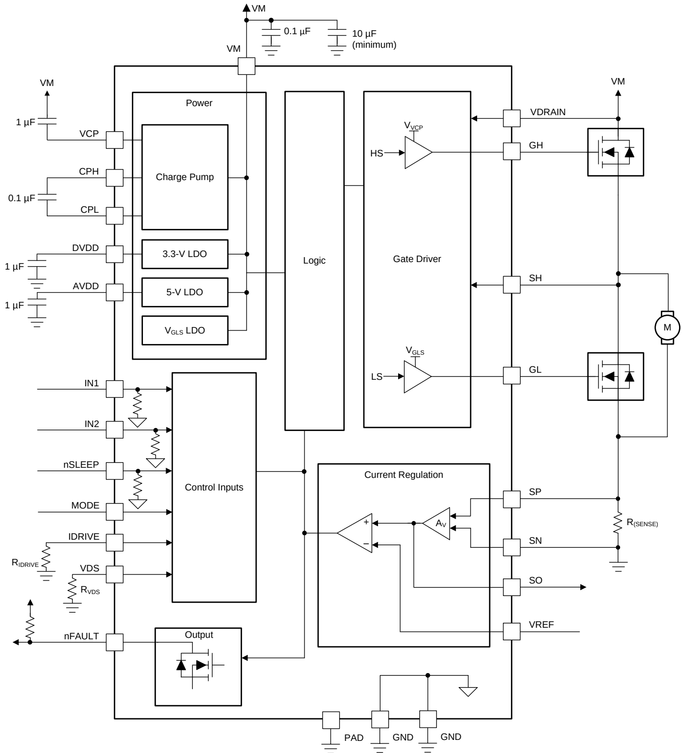
Figure 29. DRV8702D-Q1 Functional Block Diagram
