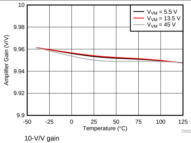
Figure 11. Amplifier Gain
