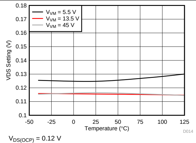
Figure 16. OCP Threshold Voltage
