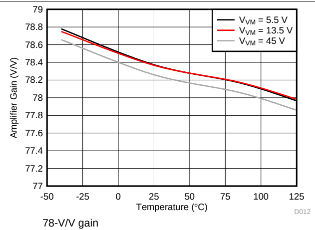
Figure 14. Amplifier Gain
