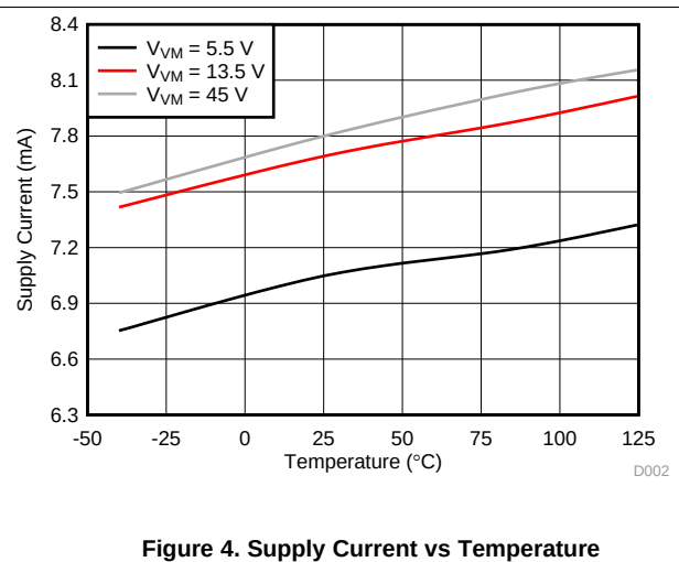
Figure 4. Supply Current vs Temperature
