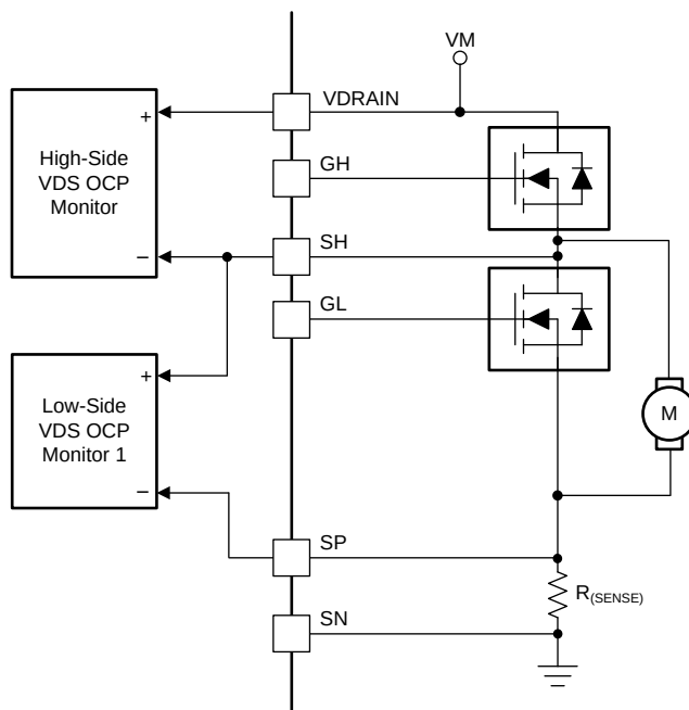
Figure 41. V_{DS(OC)} Block Diagram
