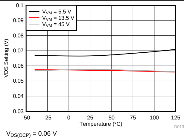
Figure 15. OCP Threshold Voltage
