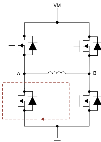
Figure 7-7. Brake Operation (Slow Decay)
