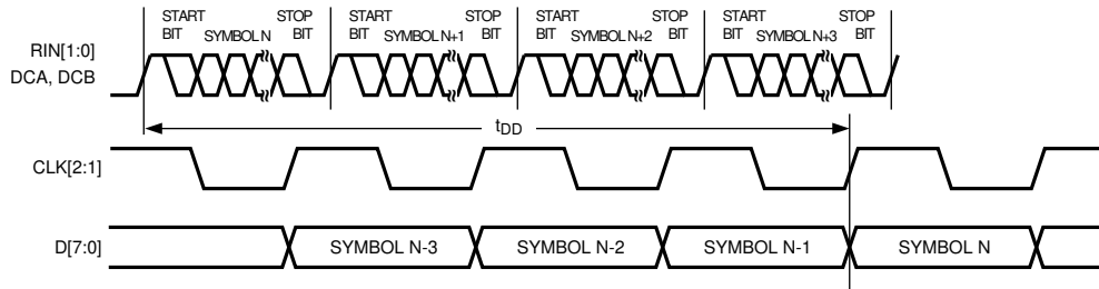
Figure 6-4. Latency Delay
