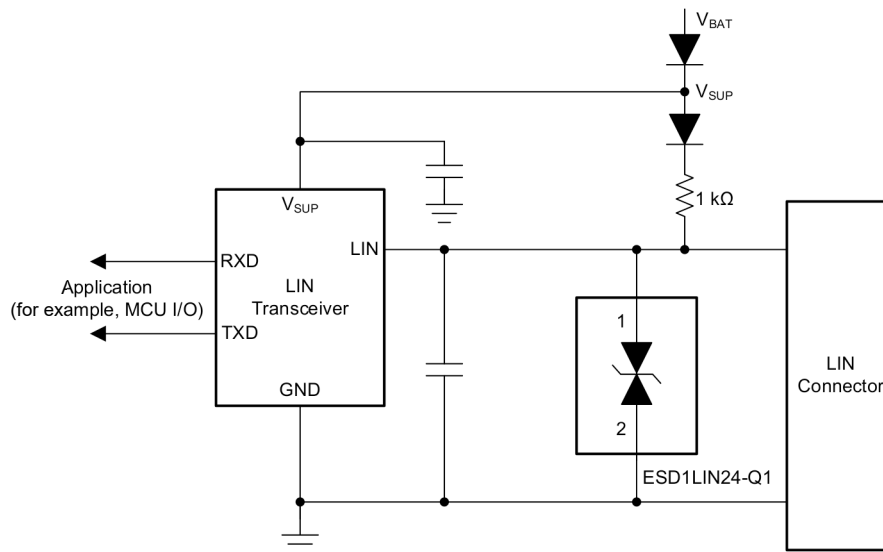
Figure 7-1. Typical Application
