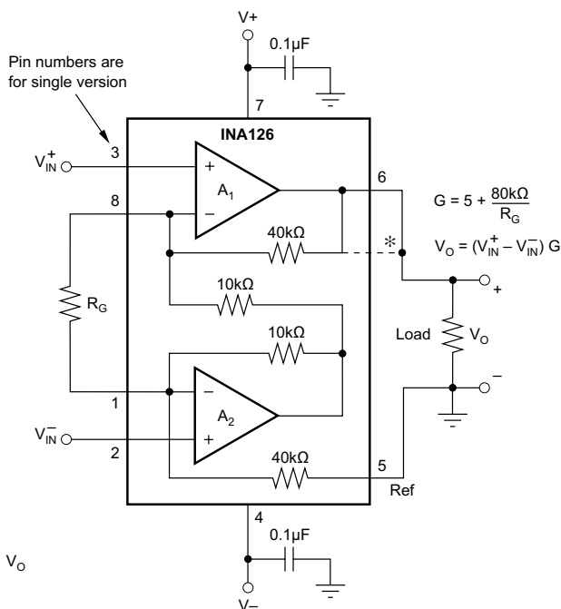
Figure 7-1. Basic Connections
