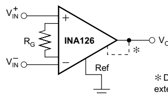
Figure 7-1. Basic Connections
