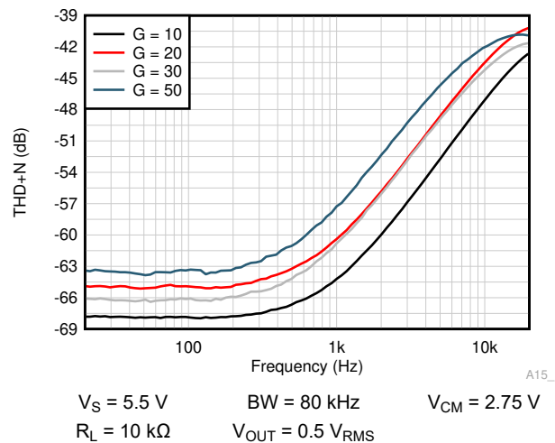
Figure 7-36. THD + N Frequency
