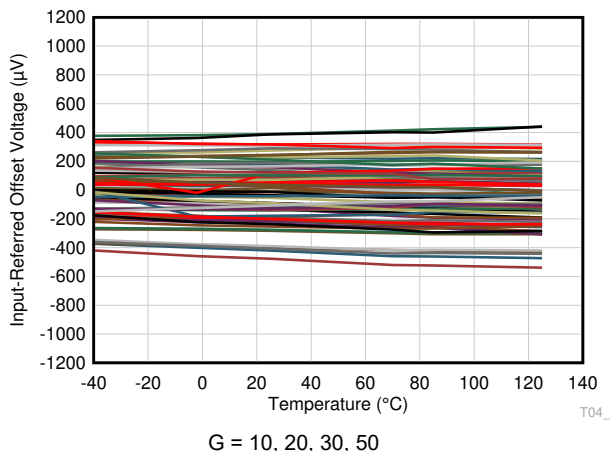
Figure 7-11. Input Referred Offset Voltage vs Temperature
