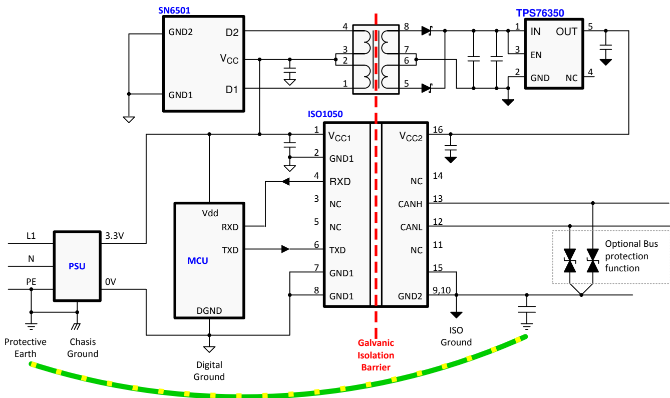
Figure 9-1. Application Circuit
