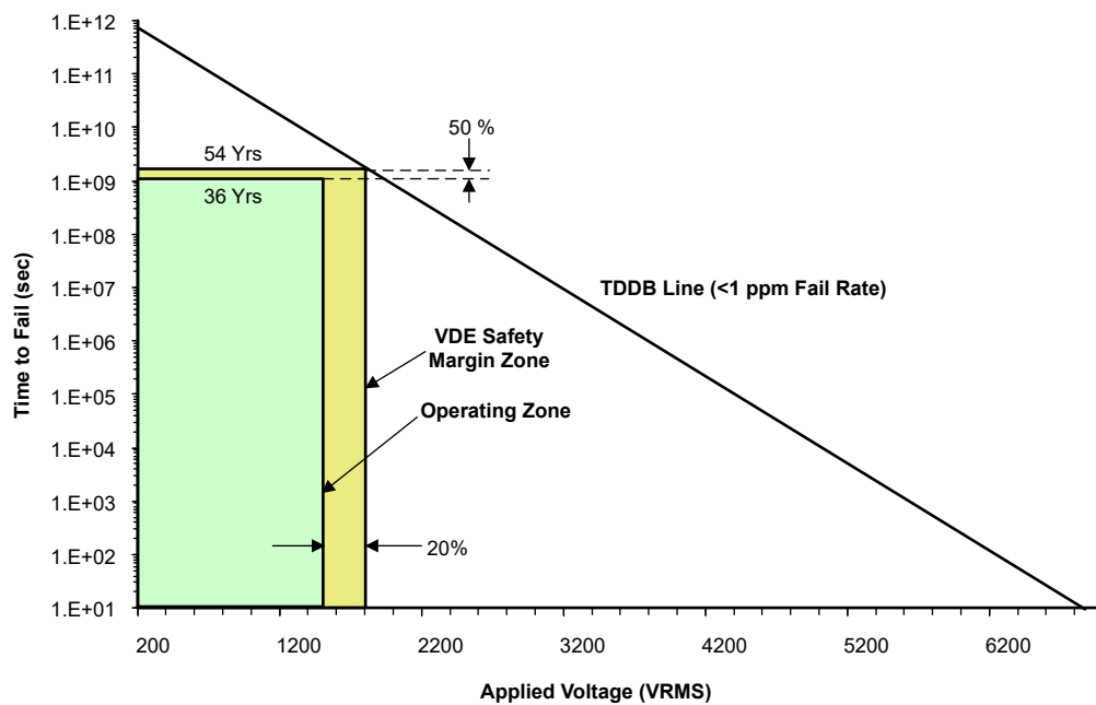
Figure 9-6. Insulation Lifetime Projection Data
