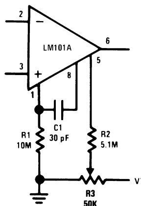
Figure 38. Standard Compensation and Offset Balancing Circuit
