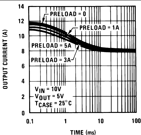
Figure 3. Current Limit
