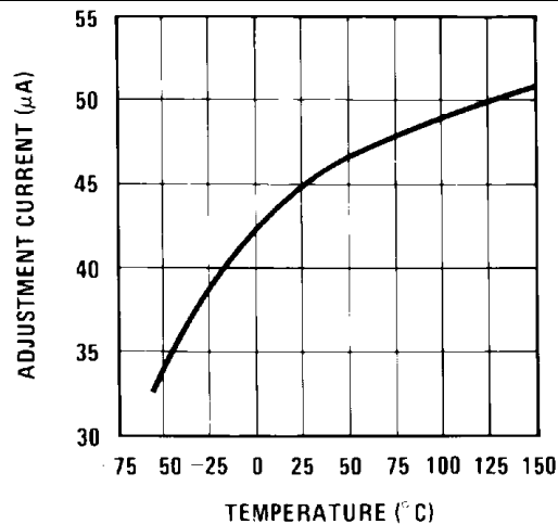
Figure 6. Adjustment Current
