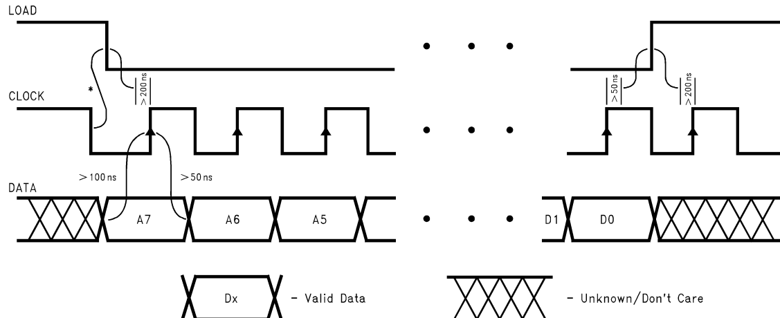
Figure 15. Timing Diagram
