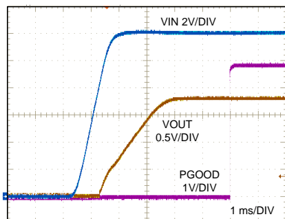
Figure 31. Startup
