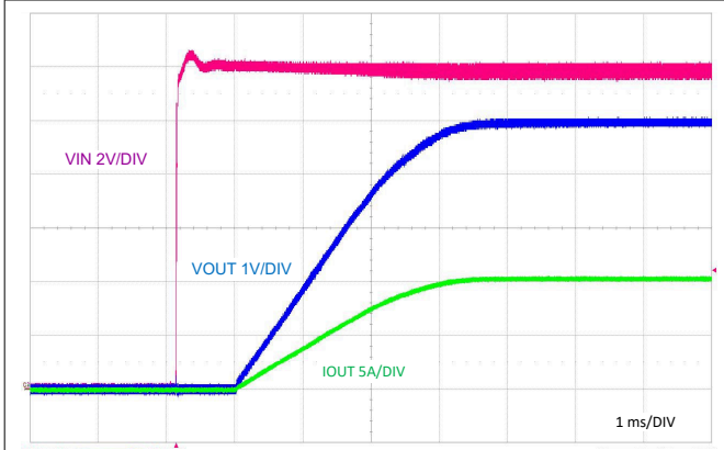
V_{IN} step to 12 V 10-A resistive load Figure 9-24. Start-Up Characteristic
