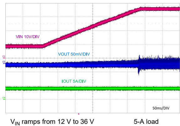
Figure 9-9. Line Transient
