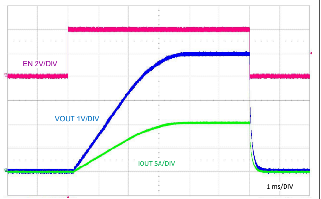
V_{IN} = 12 V 10-A resistive load Figure 9-25. ENABLE ON and OFF Characteristic
