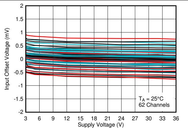
Figure 2-12. Input Offset Voltage vs. Supply Voltage at 25^\circ\text{C}
