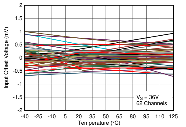
Figure 2-10. Input Offset Voltage vs. Temperature at 36V
