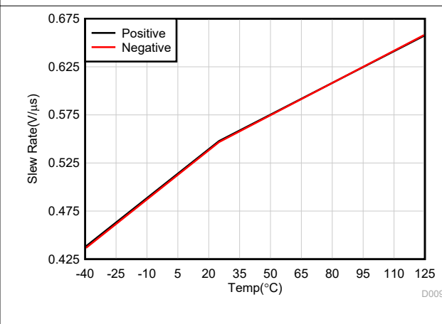
Figure 5-34. Slew Rate vs Temperature
