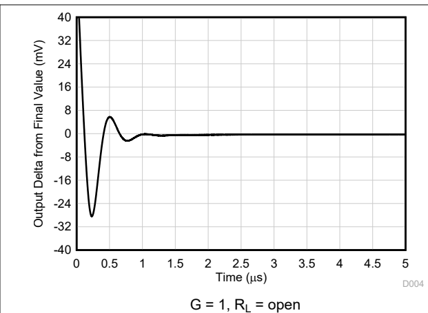
Figure 5-32. Large-Signal Step Response (Falling)
