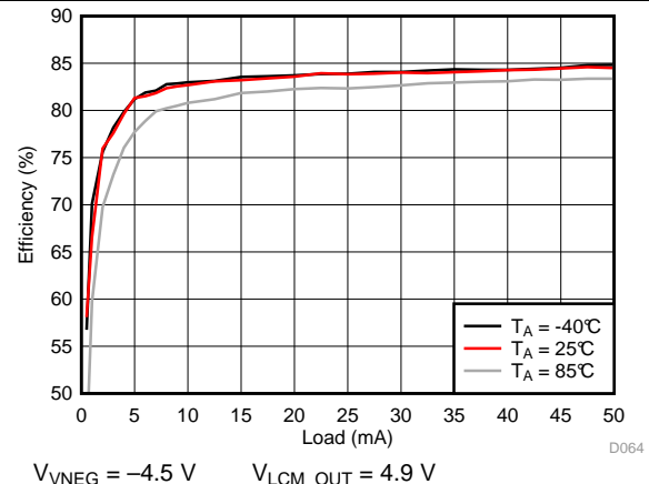
Figure 85. VNEG Efficiency
