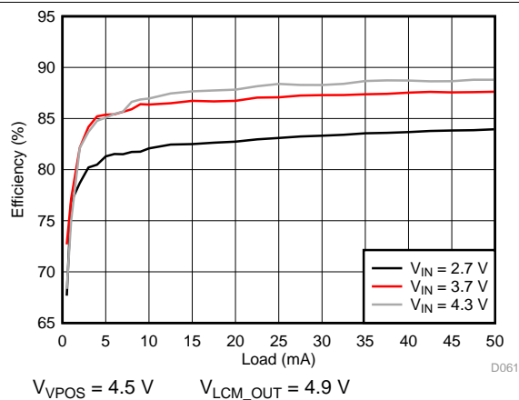
Figure 82. VPOS Efficiency
