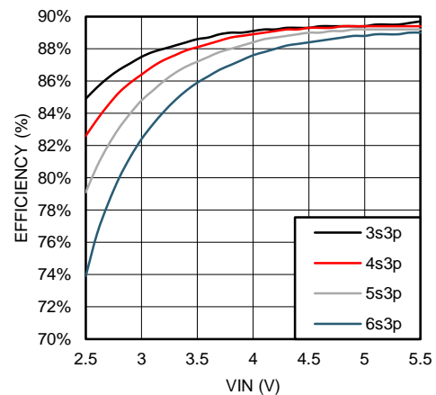
Boost Efficiency vs VIN with 10-μH Inductor
