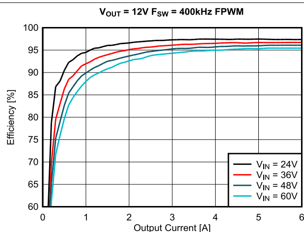
Figure 9-5. FPWM Mode Efficiency, Linear Scale
