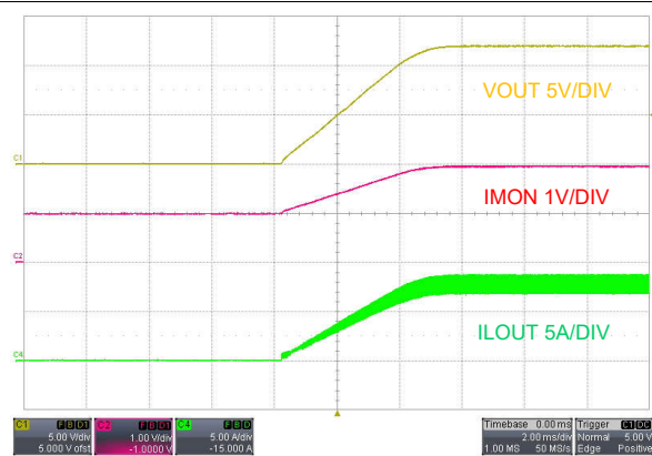
Figure 9-7. Start-Up, EN ON, V_{SUPPLY} = 48V , I_{LOAD} = 8A Resistive Load
