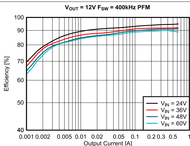
Figure 9-6. PFM Mode Efficiency, Log Scale
