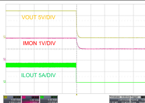
Figure 9-8. Shutdown, EN OFF, V_{SUPPLY} = 48V , I_{LOAD} = 8A Resistive Load
