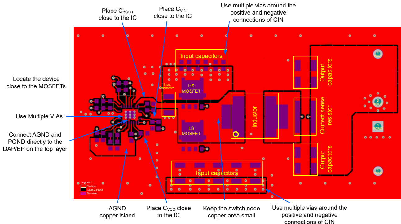
Figure 9-16. PCB Top Layer
