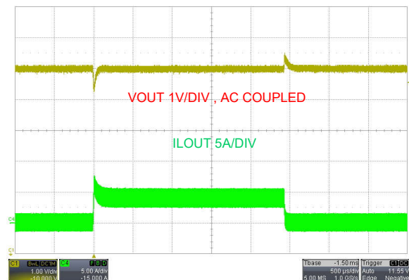
Figure 9-11. Load Transient Response, V_{\text{SUPPLY}} = 48\text{V} , FPWM, 0A to 4A
