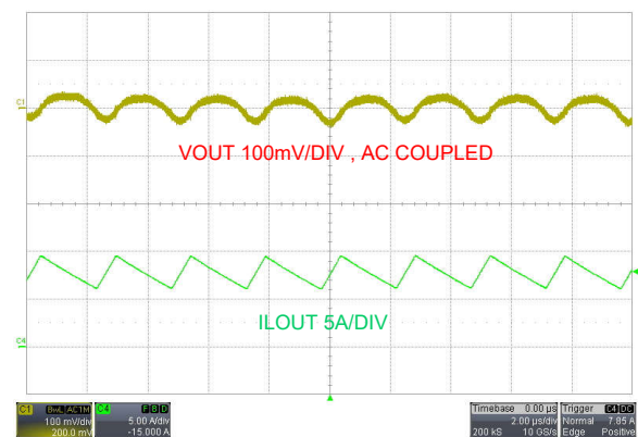
Figure 9-9. Output Ripple, V_{SUPPLY} = 48V , I_{LOAD} = 8A
