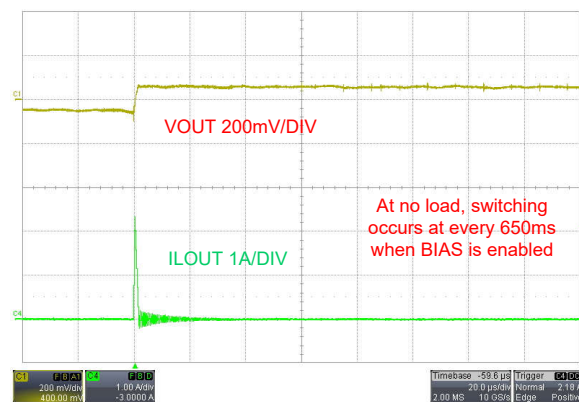
Figure 9-10. No Load Operation in PFM Mode, V_{SUPPLY} = 48V , I_{LOAD} = 0A
