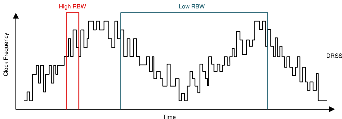
Figure 7-2. Dual Random Spread Spectrum Implementation
