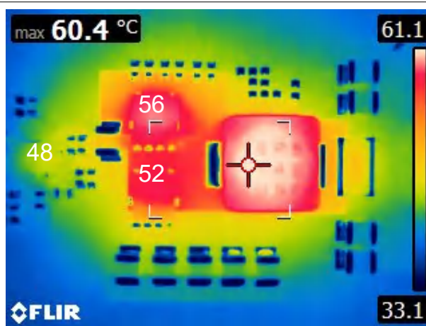
Figure 9-14. V_{\text{SUPPLY}} = 48\text{V} , I_{\text{LOAD}} = 8\text{A} , T_A = 25^\circ\text{C} , No Airflow
