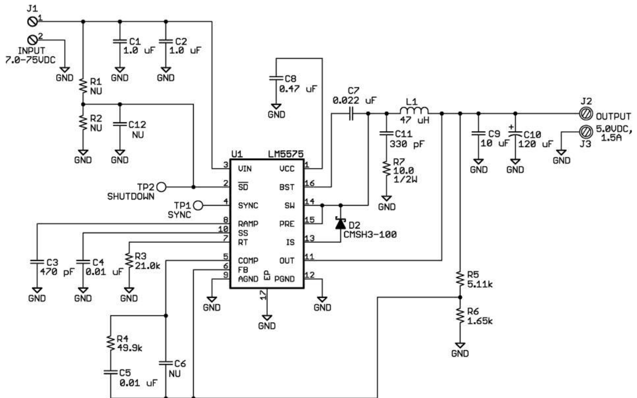
Figure 7-3. Schematic Diagram
