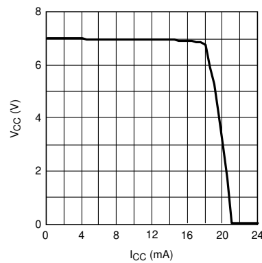
Figure 5-4. V_{cc} vs I_{cc} V_{in} = 12V
