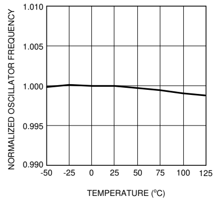
Figure 5-2. Oscillator Frequency VS Temperature F_{osc} = 200kHz
