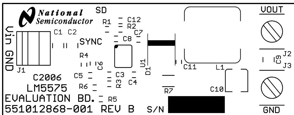
Figure 7-14. Silkscreen
