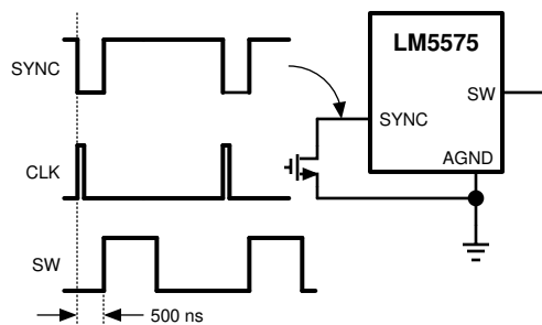
Figure 6-2. Sync From External Clock
