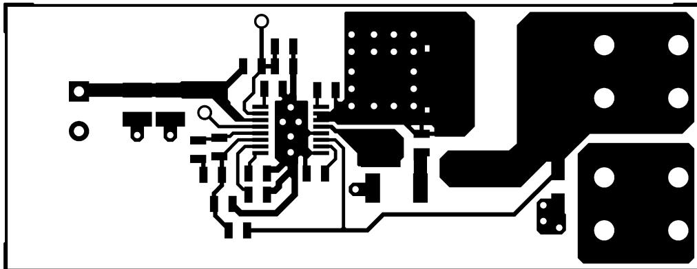
Figure 7-12. Component Side
