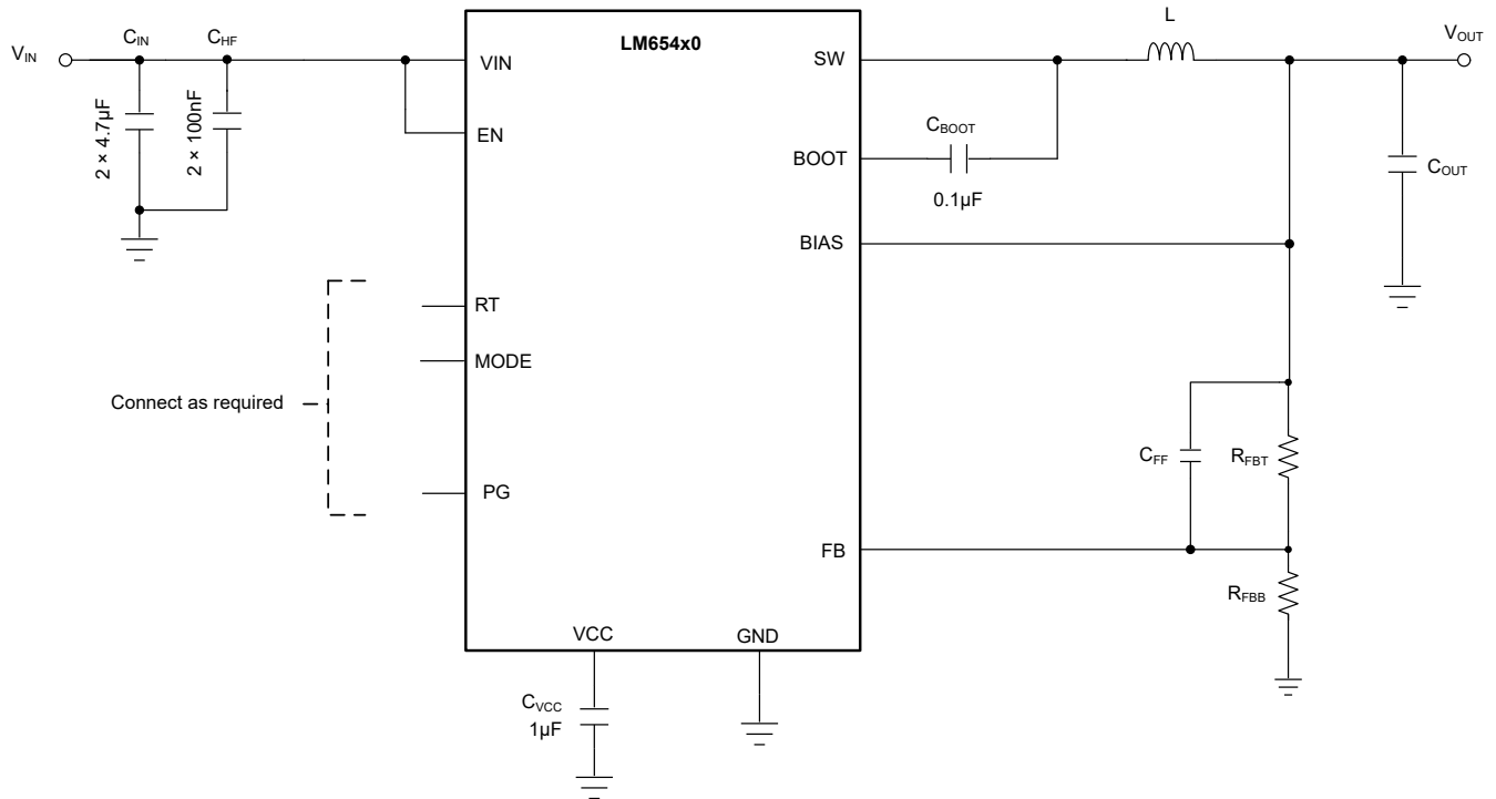
Figure 8-1. Example Application Circuit for Adjustable Output Voltage Mode With LM654x0-Q1
