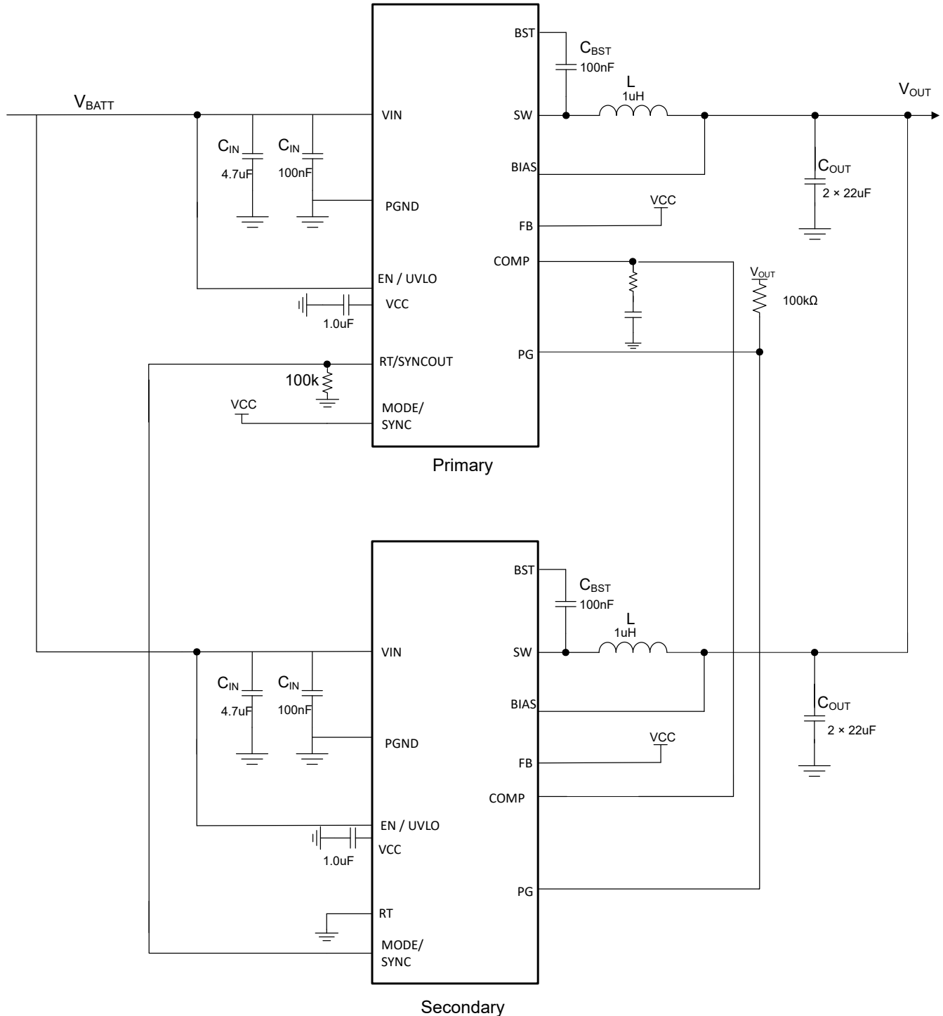
Figure 7-7. Typical fixed 5V V_{out} 2100kHz Dual Phase Schematic
