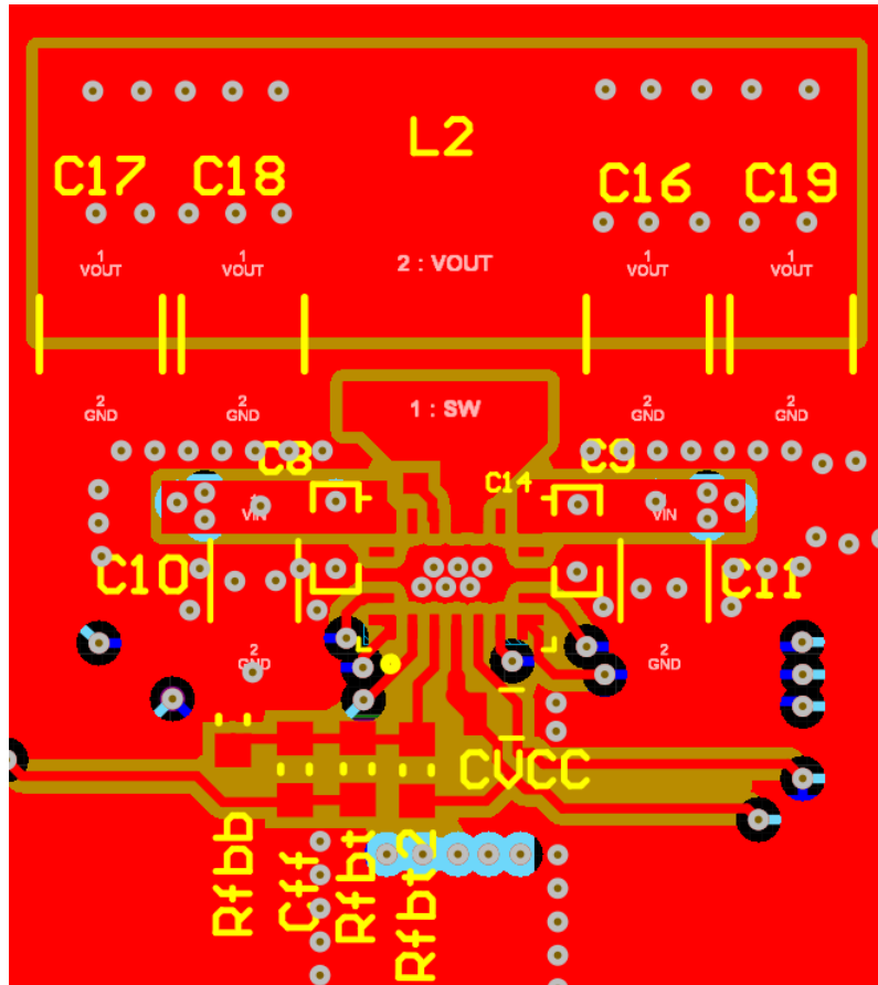
Figure 8-15. Layout Example
