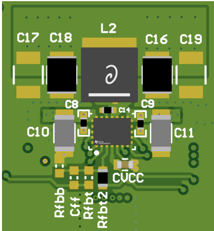
Figure 8-16. PCB Image
