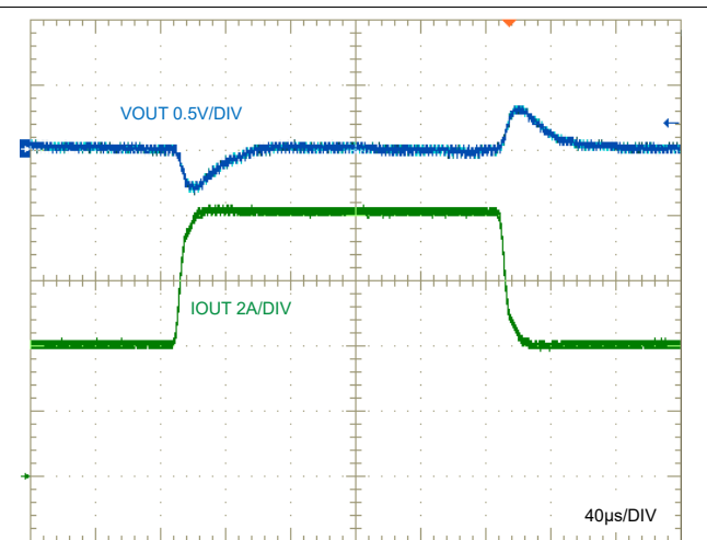
Figure 8-30. Load Transient Response, 4A to 8A
