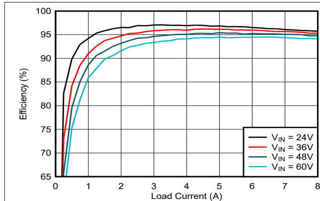
Figure 8-27. Efficiency vs I_{OUT}
