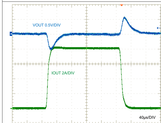
Figure 8-29. Load Transient Response, 0A to 8A
