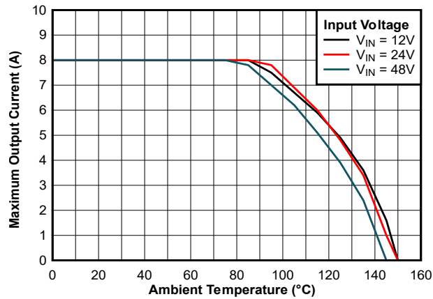
Figure 8-3. LM65680 Output Current Derating vs Ambient Temperature (5V OUT , 400kHz)
