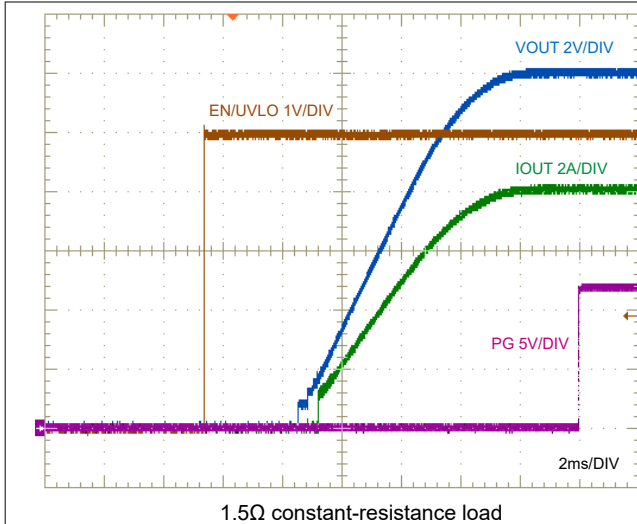
Figure 8-39. Enable ON Characteristic
