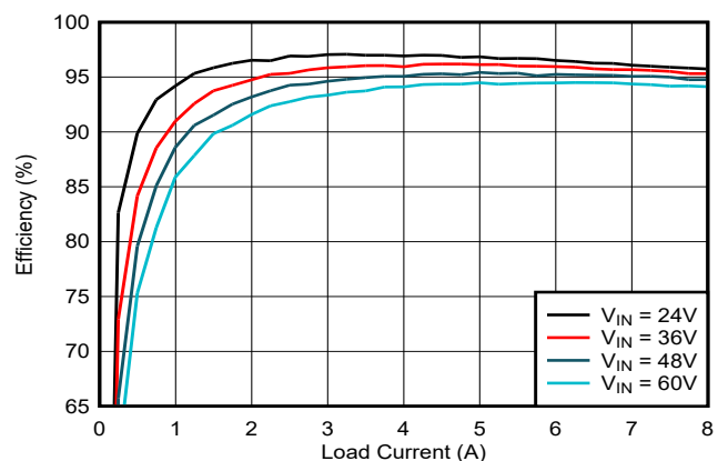
LM65680 Efficiency, V OUT = 12V, F SW = 400kHz
