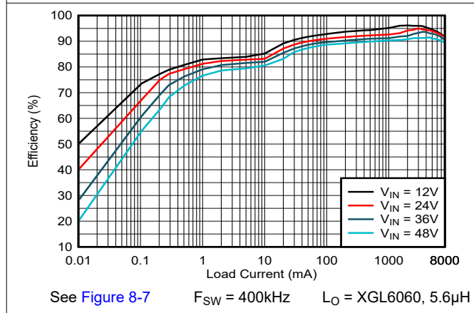
Figure 6-3. Efficiency, AUTO Mode, V_{OUT} = 5\text{V}
