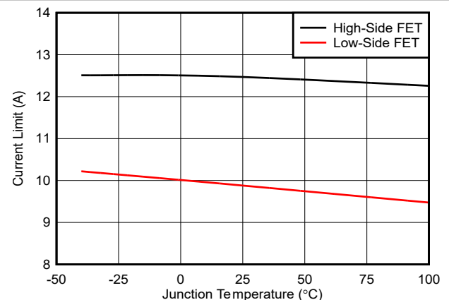
Figure 6-16. MOSFET Current Limits
