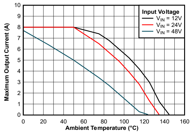
Figure 8-4. LM65680 Output Current Derating vs Ambient Temperature (12V OUT , 400kHz)
