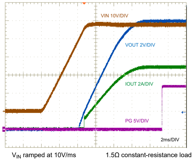
Figure 8-37. V IN Start-up Characteristic
