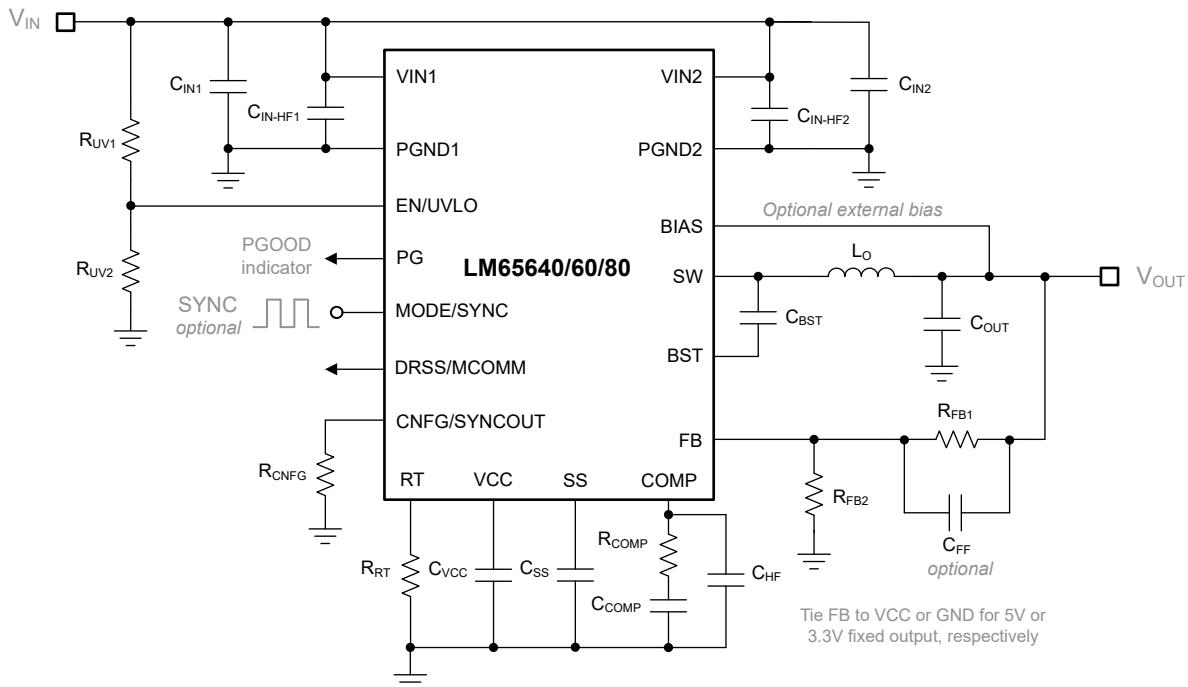
Figure 7-1. LM65680/60/40 Regulator Schematic
