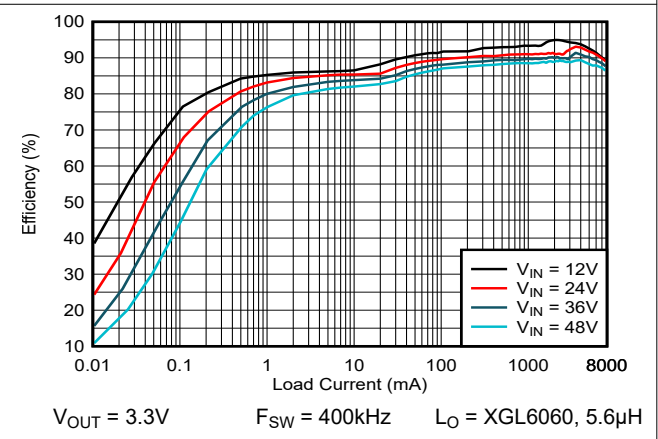
Figure 6-4. Efficiency, AUTO Mode, V_{OUT} = 3.3\text{V}
