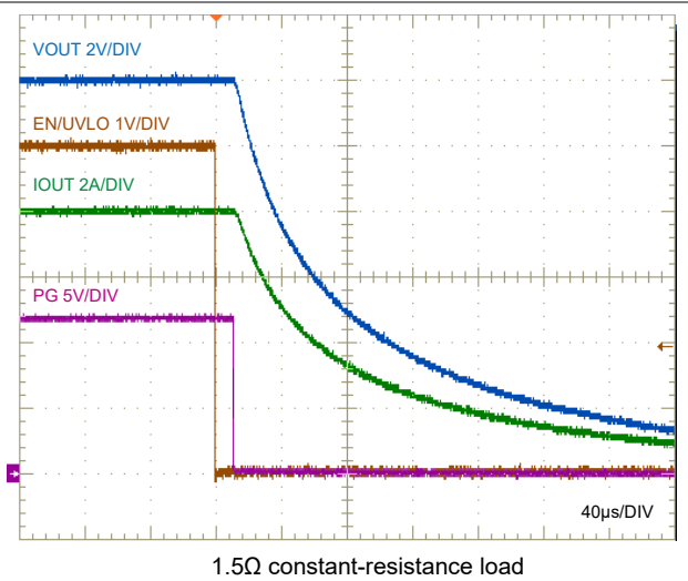
Figure 8-40. Enable OFF Characteristic
