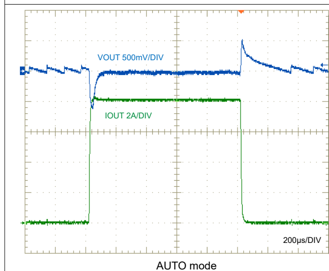
Figure 8-31. Load Transient Response, 0A to 8A
