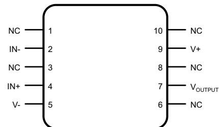
Figure 2. 10-Pin CFP Top View
