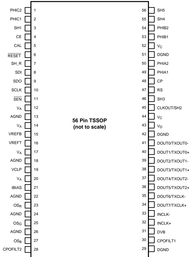
56-Pin TSSOP Package DGG056A (Top View)
