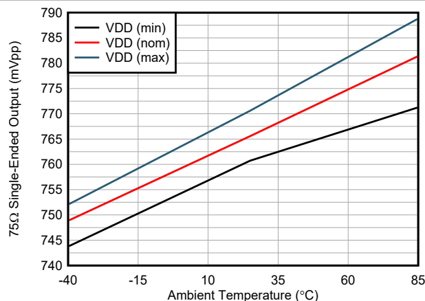
Figure 5-7. SDI_OUT VOD at 11.88Gbps
