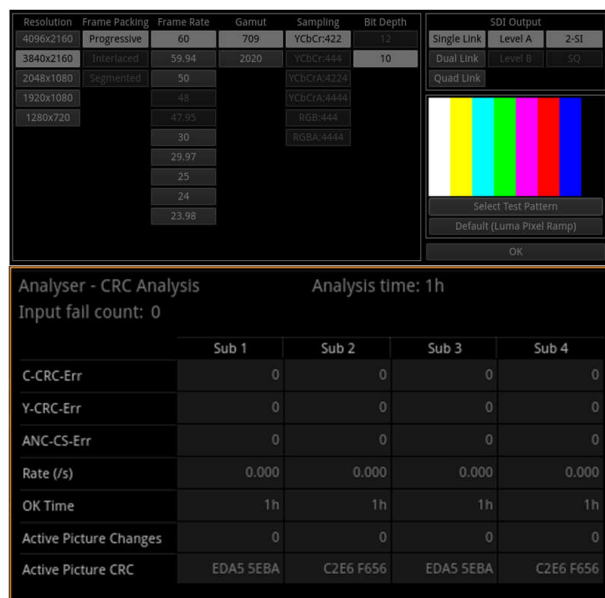
IN_MUX_SEL = F (SDI_IN selected), VOD_DE = F, SDI_OUT_SEL = H, OUT_CTRL = F Figure 7-18. OUT0± BER at 11.88Gbps (12G-SDI), CC = 100m Belden 1694A, Reclocked
