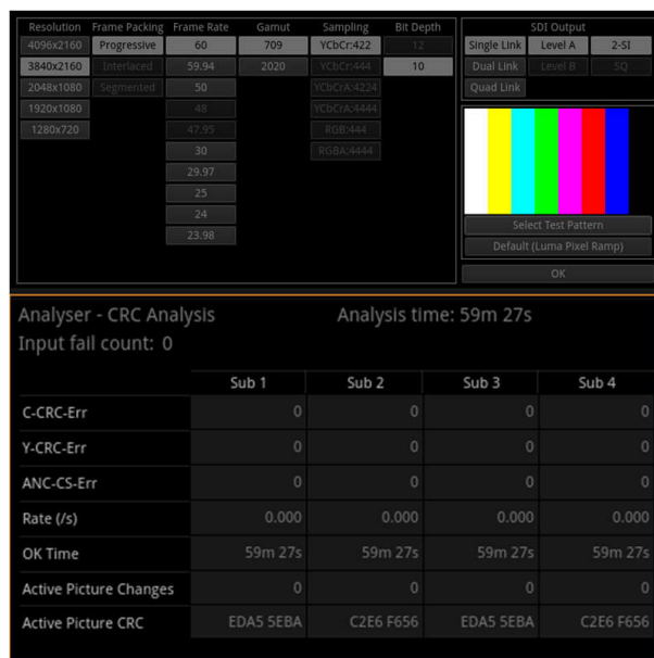
IN_MUX_SEL = L (SDI_IN1 selected), VOD_DE = F, SDI_OUT_SEL = H, OUT_CTRL = F Figure 7-19. OUT0± BER at 11.88Gbps (12G-SDI), CC = 100m Belden 1694A, Reclocked
