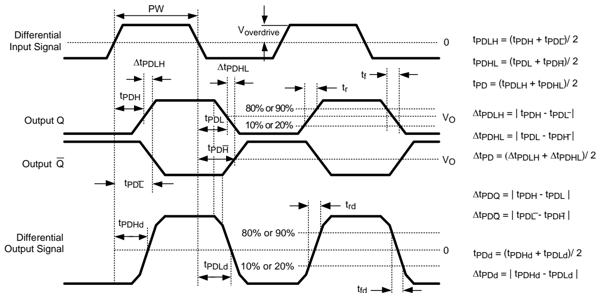
Figure 15. Timing Definitions
