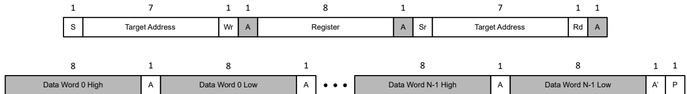
Figure 7-7. Generic Block Read Sequence
