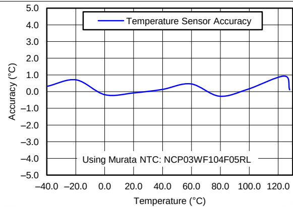
Figure 3. Temperature Accuracy
