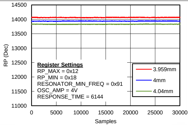
Figure 2. R_p Resolution
