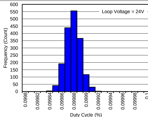
Figure 9. 0.1% Duty Cycle Distribution, NPN Mode
