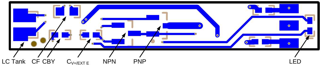
Figure 28. LMP91300 PNP Layout Example
