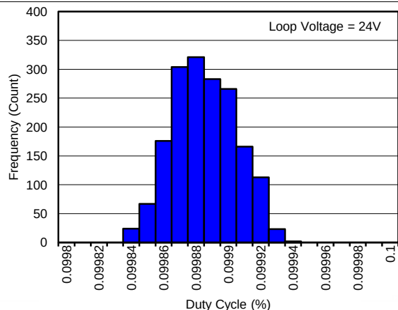
Figure 8. 0.1% Duty Cycle Distribution, PNP Mode
