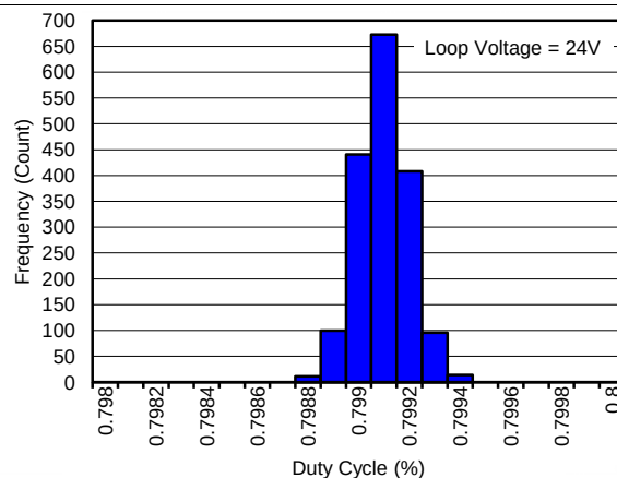
Figure 11. 0.8% Duty Cycle Distribution, NPN Mode
