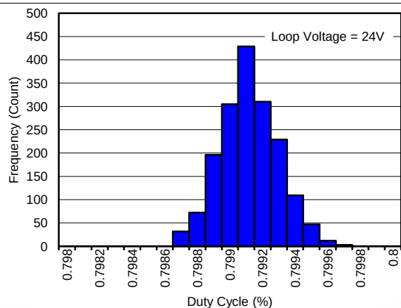
Figure 10. 0.8% Duty Cycle Distribution, PNP Mode
