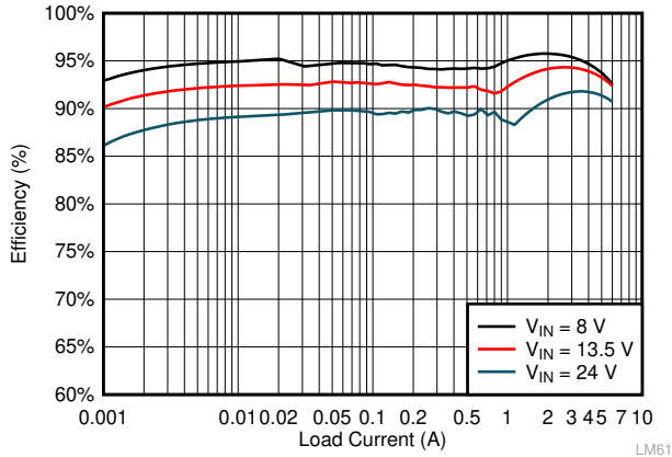
Figure 10-11. LMQ61460-Q1 Efficiency
