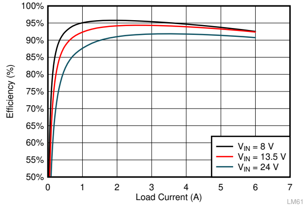
Figure 10-12. LMQ61460-Q1 Efficiency
