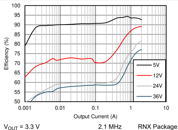
Figure 9-18. Efficiency
