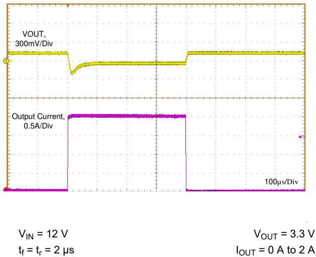
Figure 9-29. Load Transient
