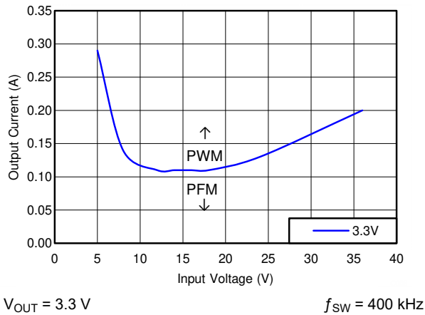
Figure 9-27. Mode Change Thresholds
