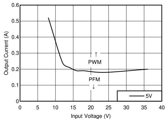
Figure 9-11. Mode Change Thresholds
