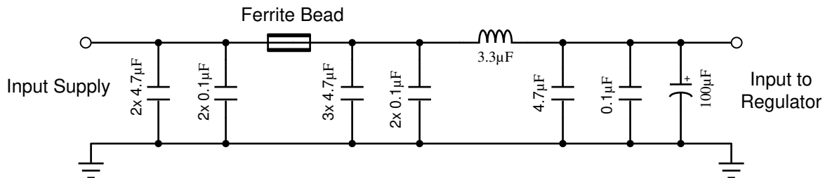
Figure 9-28. Typical Input EMI Filter Filter Used Only for EMI Measurements Found in Application Curves
