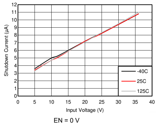
Figure 7-2. Shutdown Supply Current
