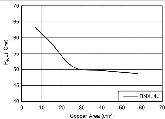
Figure 9-3. R_{\theta JA} vs Copper Board Area for the VQFN (RNX) Package
