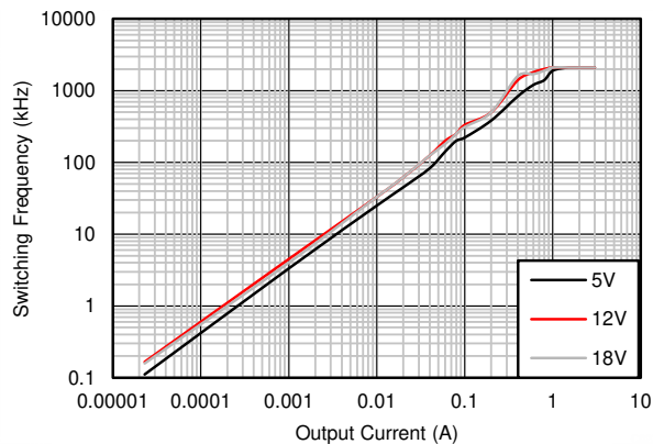
Figure 9-18. Switching Frequency vs Output Current
