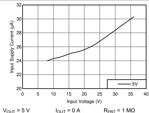
Figure 9-10. Input Supply Current
