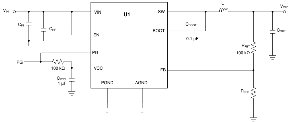
Figure 9-27. Circuit for Application Curves
