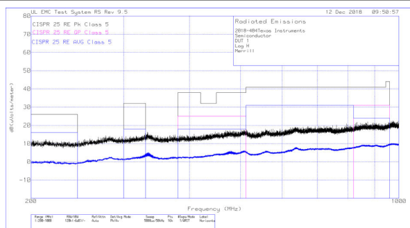
Figure 9-24. Radiated EMI Log-Periodic Antenna (Horizontal)
