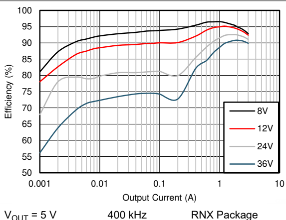
Figure 9-5. Efficiency
