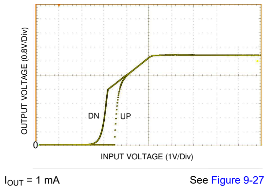
Figure 7-5. UVLO Thresholds
