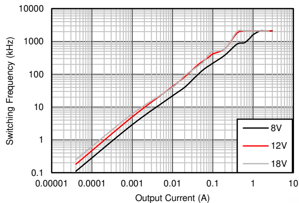
Figure 9-12. Switching Frequency vs Output Current
