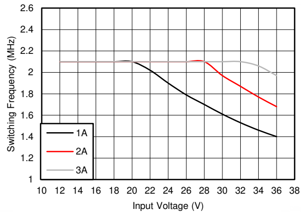
Figure 8-13. Switching Frequency vs Input Voltage V_{OUT} = 3.3\text{ V}
