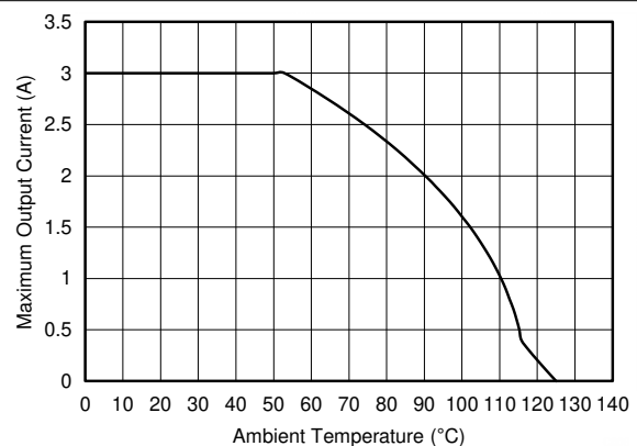
Figure 9-4. Maximum Output Current vs Ambient Temperature
