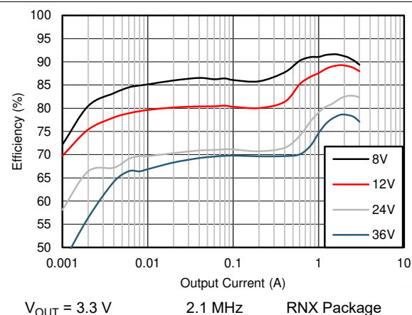
Figure 9-8. Efficiency
