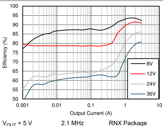
Figure 9-7. Efficiency
