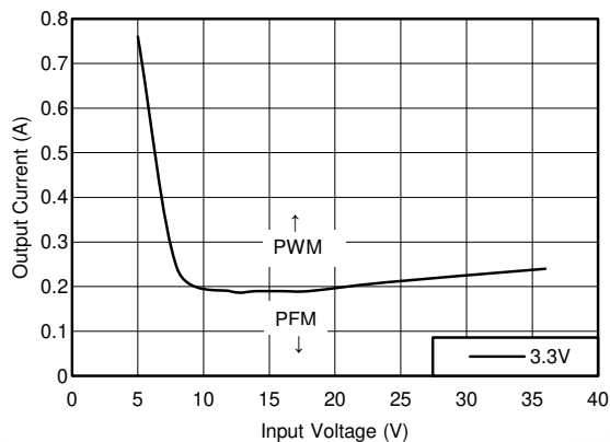
Figure 9-17. Mode Change Thresholds
