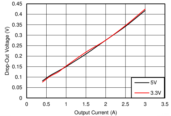
Figure 8-10. Typical Dropout Voltage vs Output Current in Frequency Foldback f_{SW} = 140\text{ kHz}
