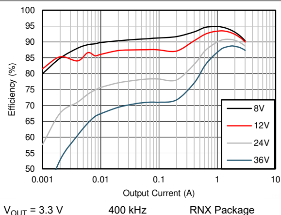
Figure 9-6. Efficiency
