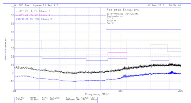
Figure 9-23. Radiated EMI Biconical Antenna (Vertical)
