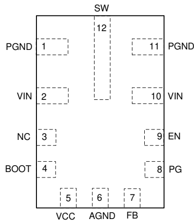
Figure 6-1. 12-Pin VQFN RNX Package (Top View)
