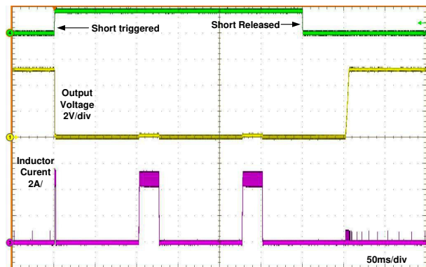
Figure 8-6. Short-Circuit Transient and Recovery
