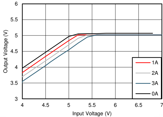
Figure 8-9. Overall Dropout Characteristic V_{OUT} = 5\text{ V}
