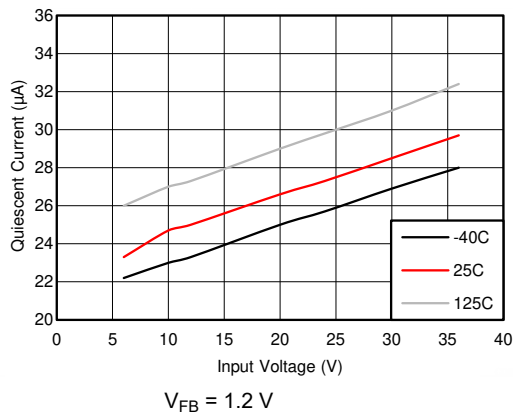
Figure 7-1. Non-Switching Input Supply Current
