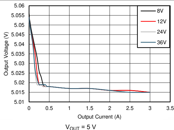
Figure 9-9. Line and Load Regulation
