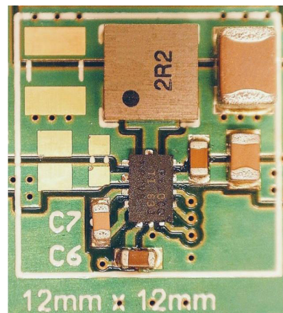
Minimum Component Example
