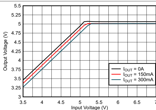
Figure 8-13. Dropout
