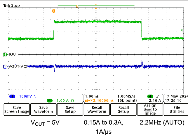
Figure 8-15. Load Transient
