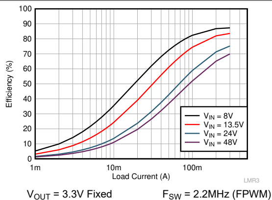
Figure 6-1. Efficiency 3.3V Output, FPWM
