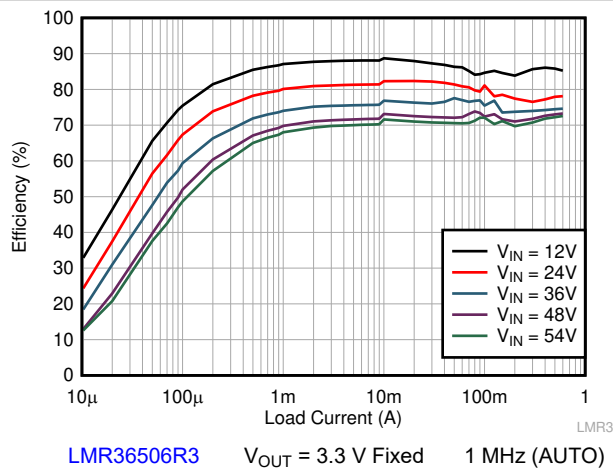
Figure 8-4. Efficiency
